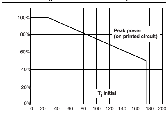
Figure 3. Peak pulse power dissipation versus initial junction temperature (printed circuit board)
