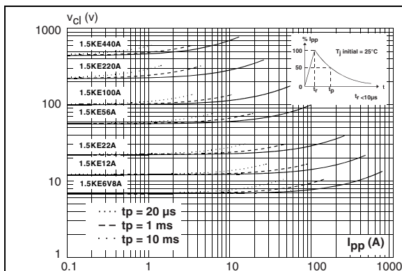
Figure 5. Clamping voltage versus peak pulse current
