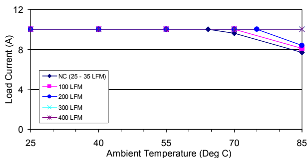
Figure 32. EMS10DG, Vin = 48 VDC
