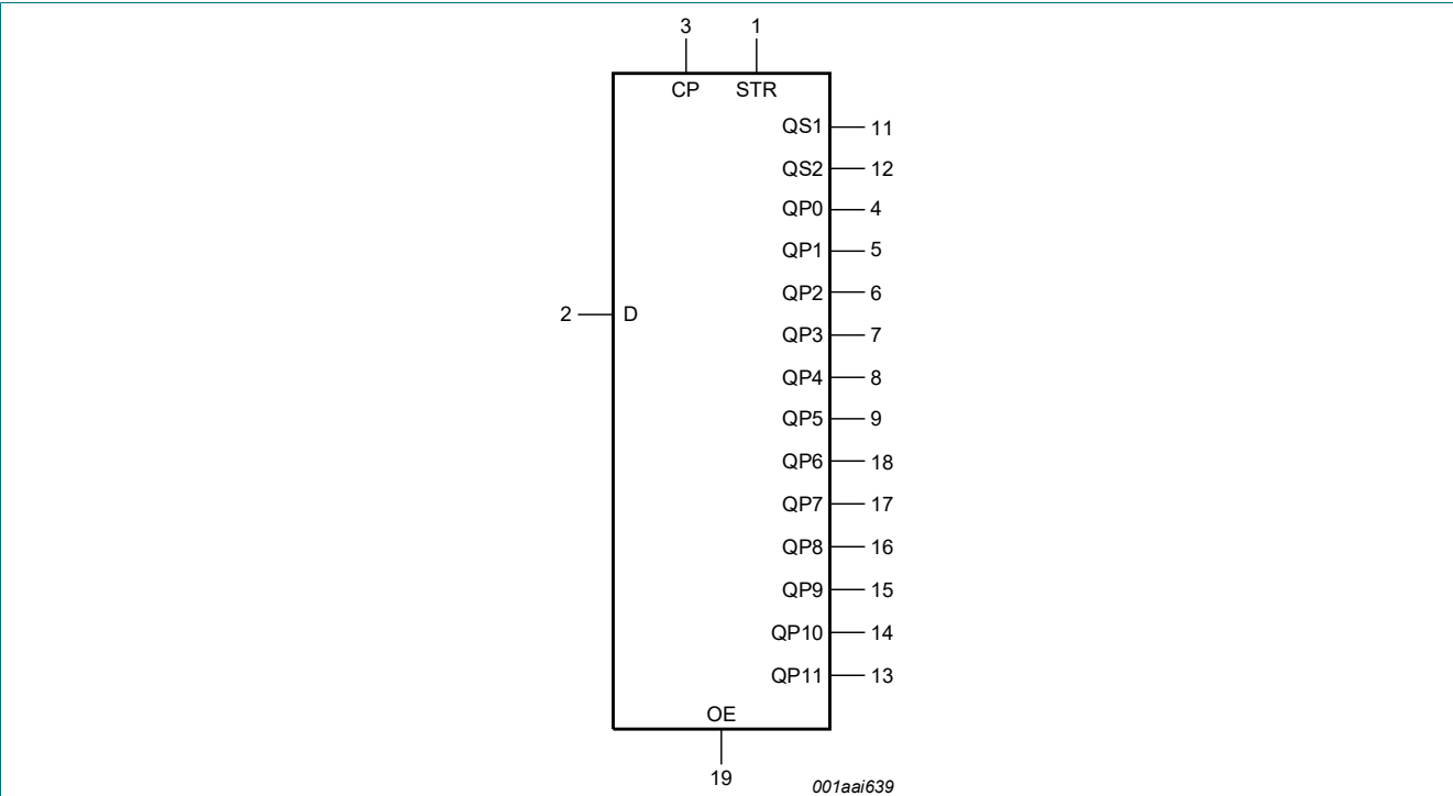
Fig. 1. Logic Symbol
