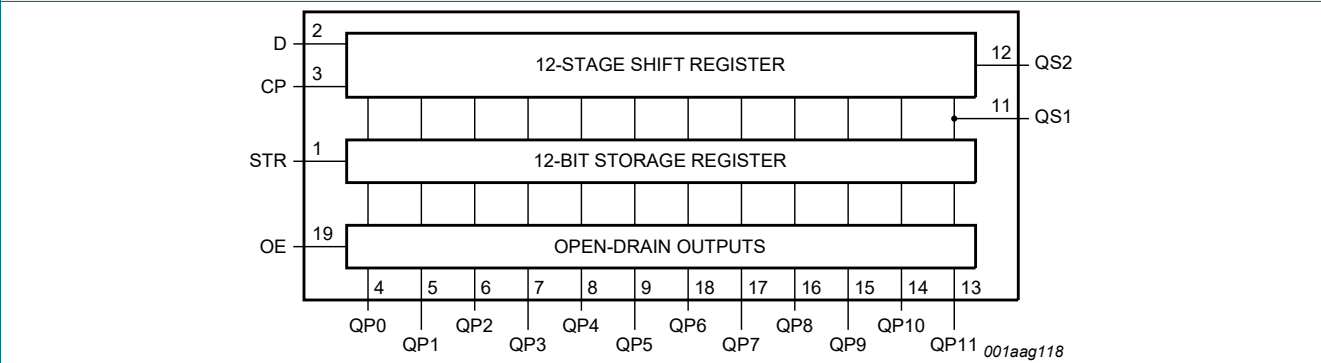
Fig. 2. Functional diagram
