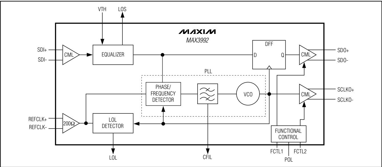
Figure 3. Functional Diagram
