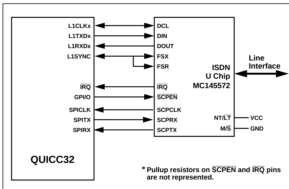
Figure C-3. IDL and SCP Connections between the QUICC32 and the U Interface
