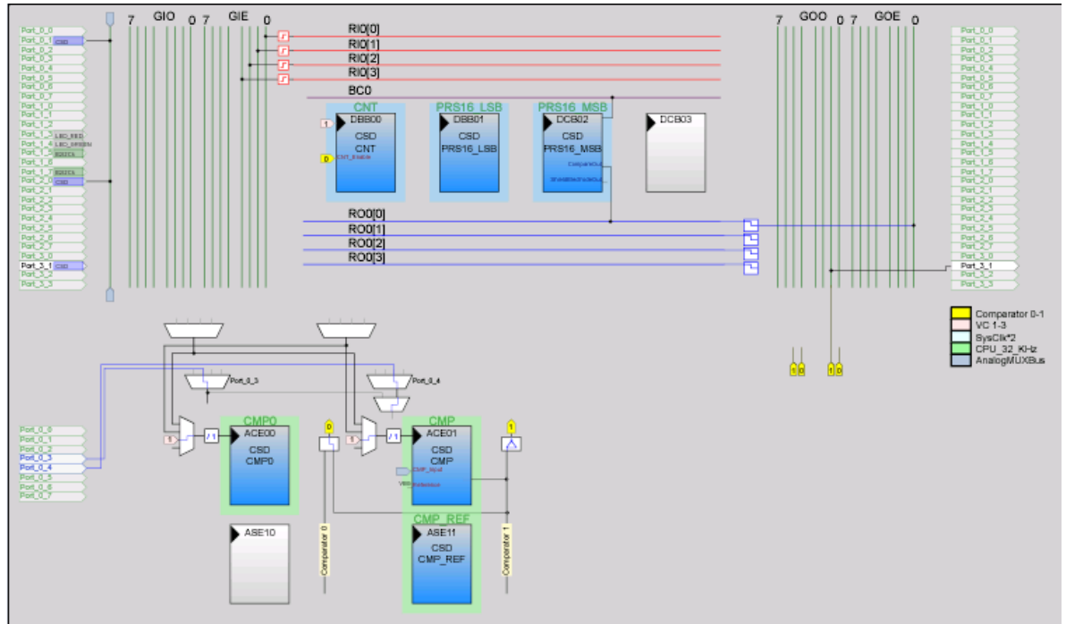
Figure 5-39. Device Configuration of Proximity Sensor
