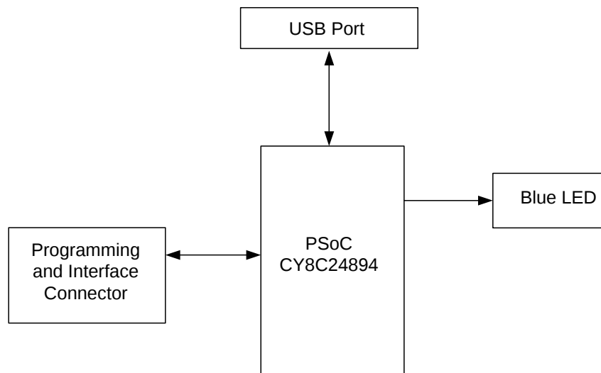
Figure 4-1. System Block Diagram for FirstTouch PC Bridge (FTPC Bridge)
