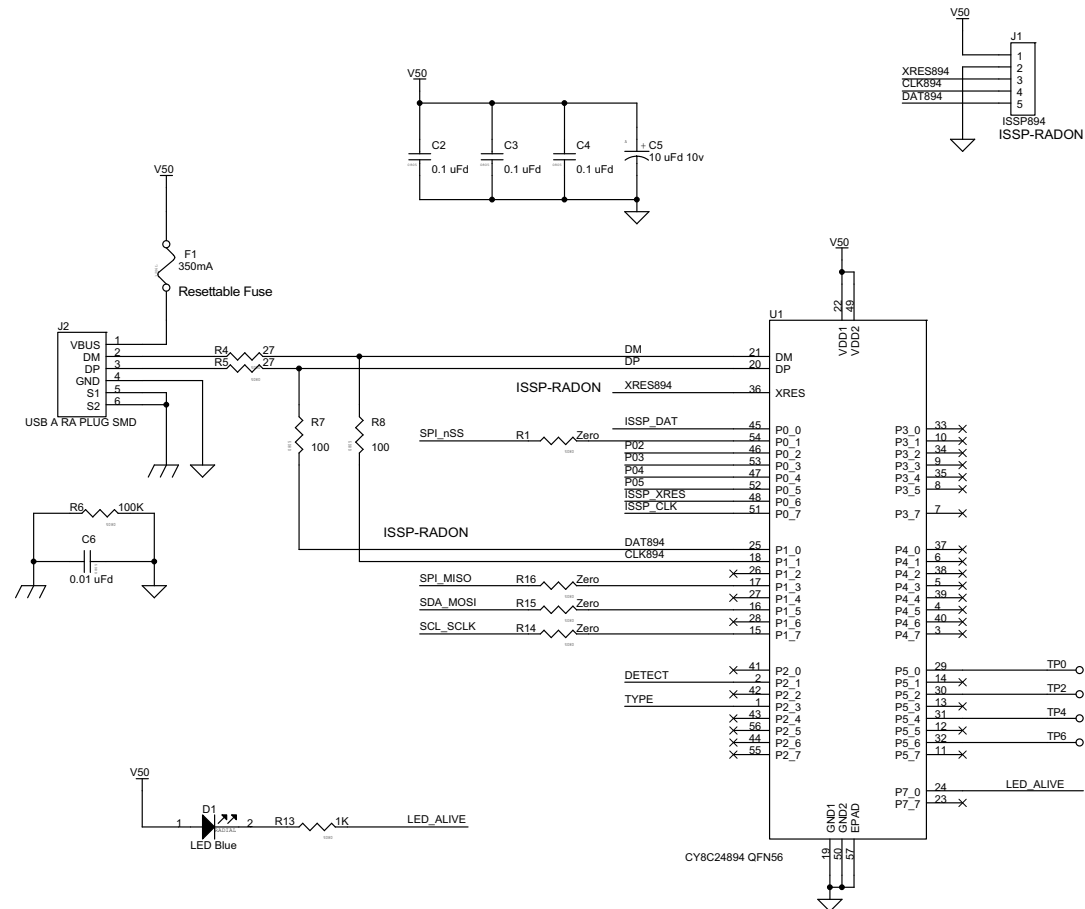
Figure 4-3. CY8C24894 Schematic
