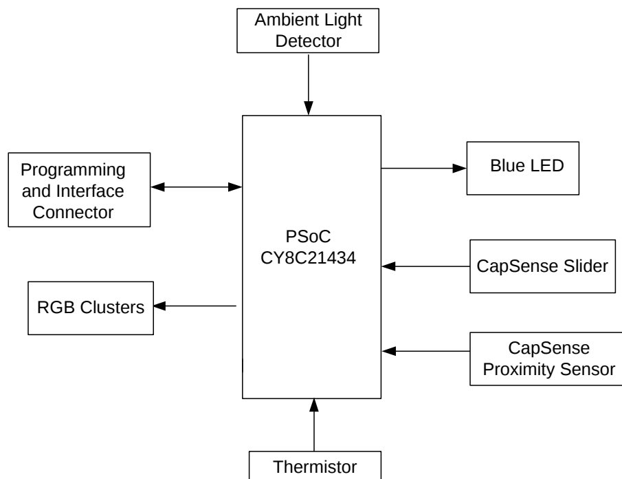
Figure 4-2. System Block Diagram for First Touch Multifunction Card
