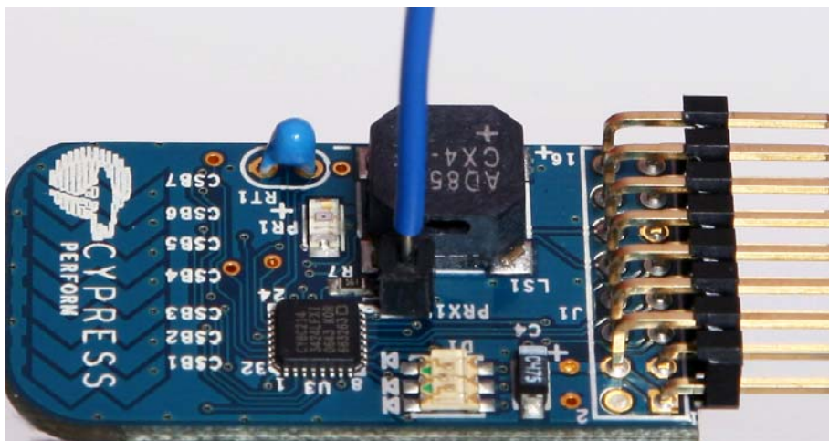
Figure 3-2. FTMF Expansion Card
