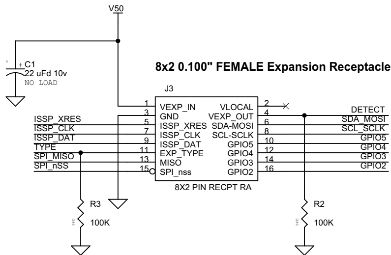
Figure 4-4. FTPC Expansion Port Pinout Diagram
