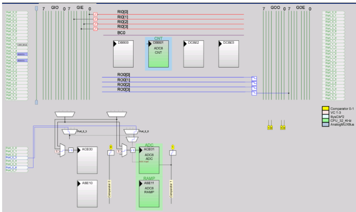
Figure 5-37. Device Configuration of Light Sensor
