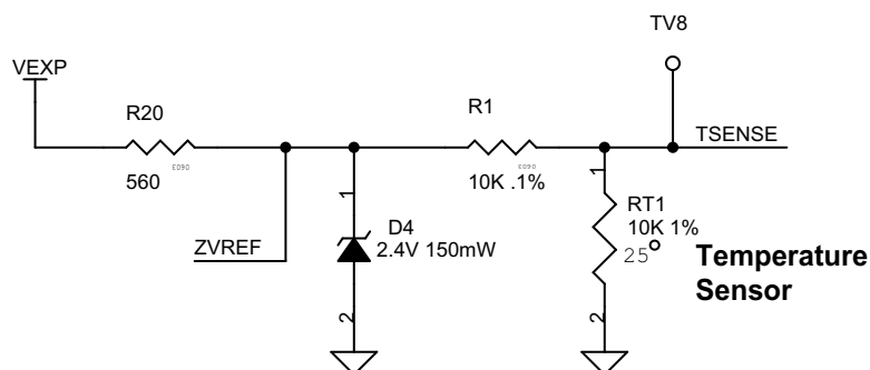
Figure 4-6. On Board Thermistor Schematic
