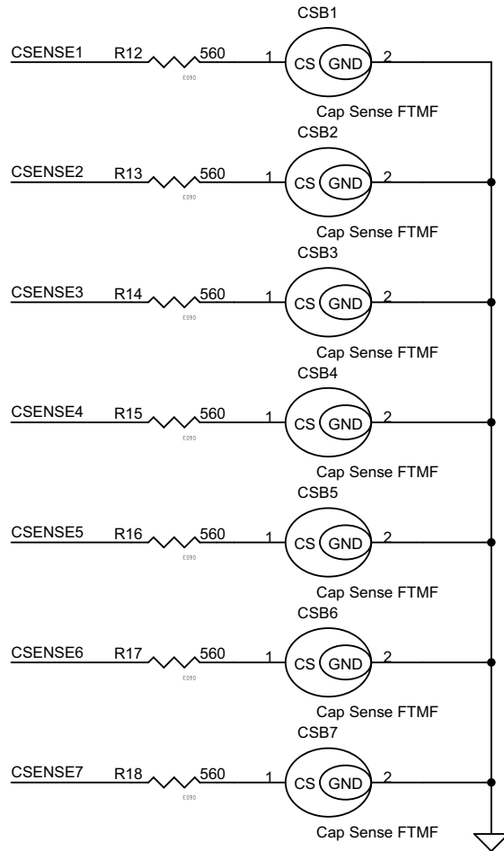
Figure 4-7. CapSense Slider Schematic
