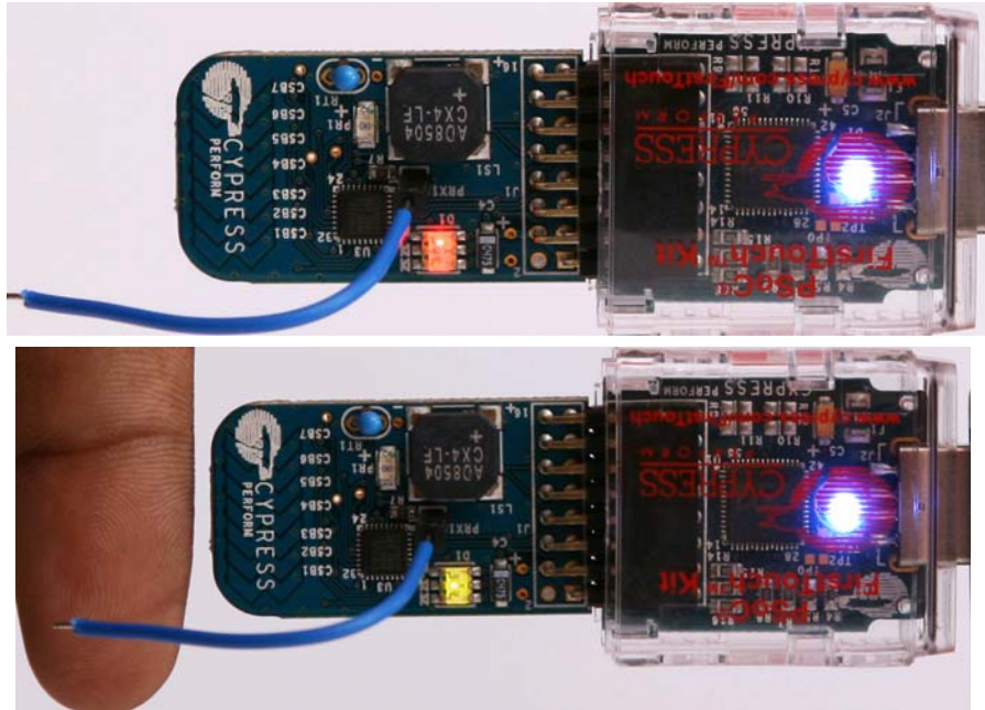
Figure 5-40. Proximity Antenna Output
