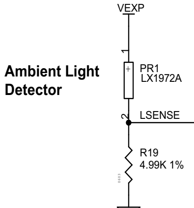
Figure 4-8. Light Sensor Schematic
