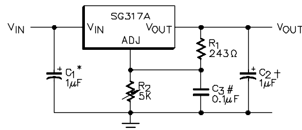
Figure 18 – Connections for Best Load Regulation
