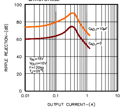
Figure 9 – Ripple Rejection vs. Output Current
