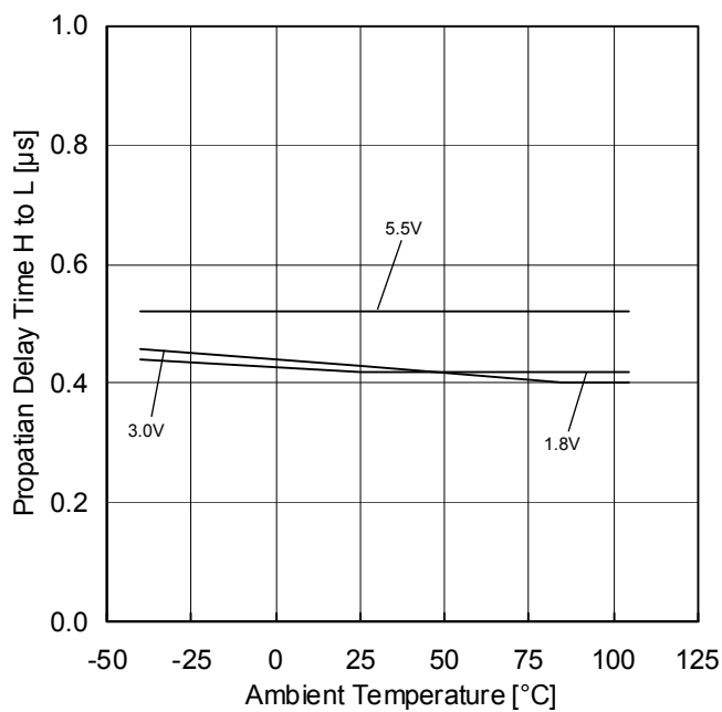
Figure 22. Propagation Delay Time H to L vs Ambient Temperature ( C_L=15\text{pF} , I_N=1.5\text{V} 100mV Overdrive)
