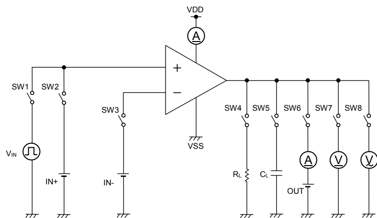
Figure 24. Test Circuit 2
