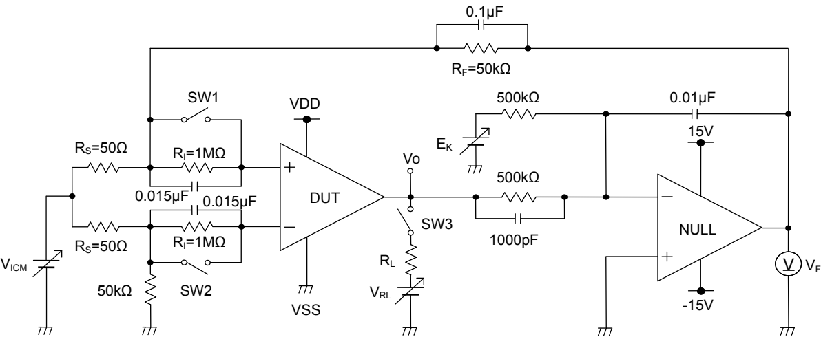
Figure 23. Test Circuit 1
