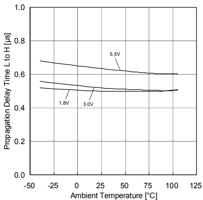
Figure 21. Propagation Delay Time L to H vs Ambient Temperature ( C_L=15\text{pF} , I_N=1.5\text{V} 100mV Overdrive)
