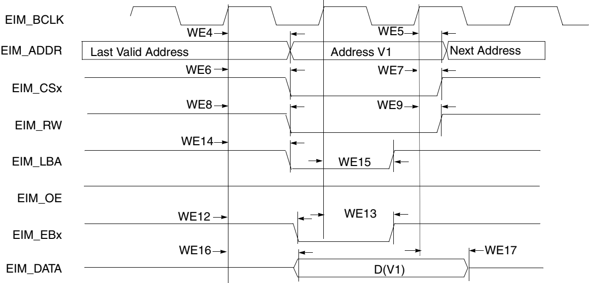
Figure 20. Synchronous Memory, Write Access, WSC=1, WBEA=1, WBEN=1, and WADVN=0
