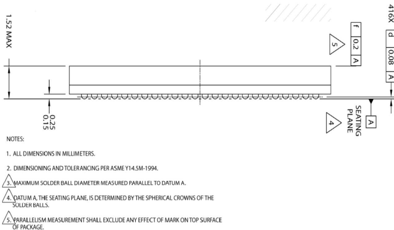
Figure 61. 416 MAPBGA 13x13 mm Package Side View
