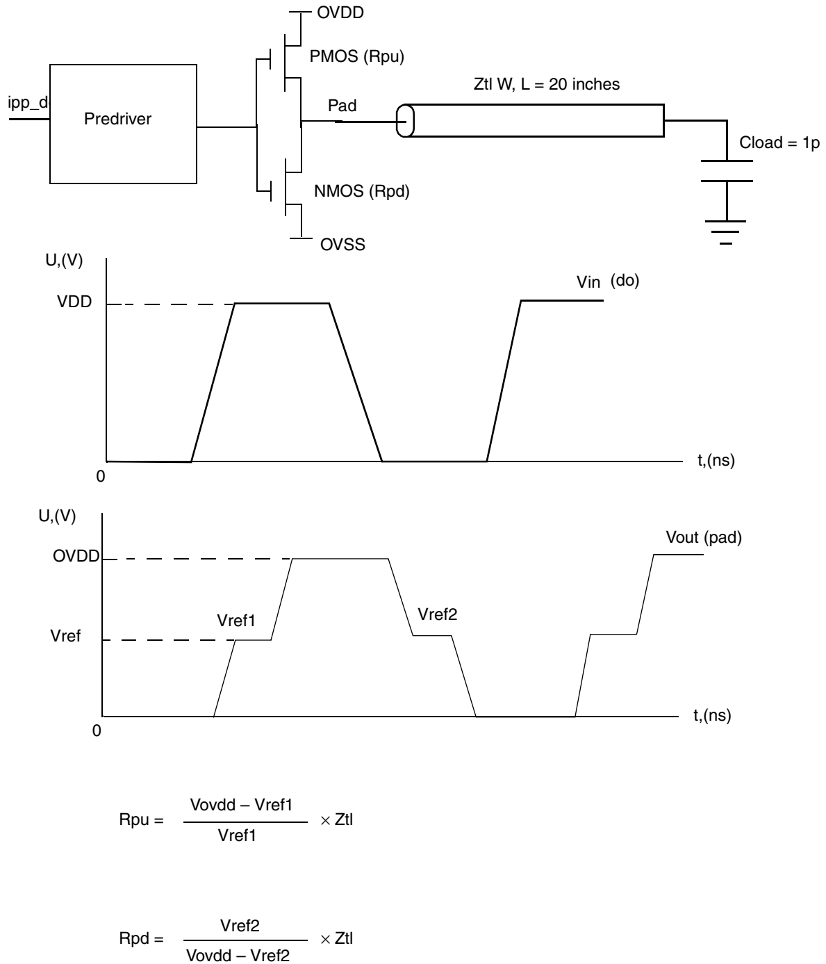
Figure 3. Impedance Matching Load for Measurement
