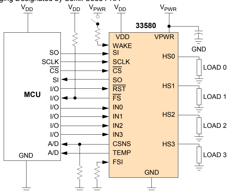
Figure 1. 33580 Simplified Application Diagram
