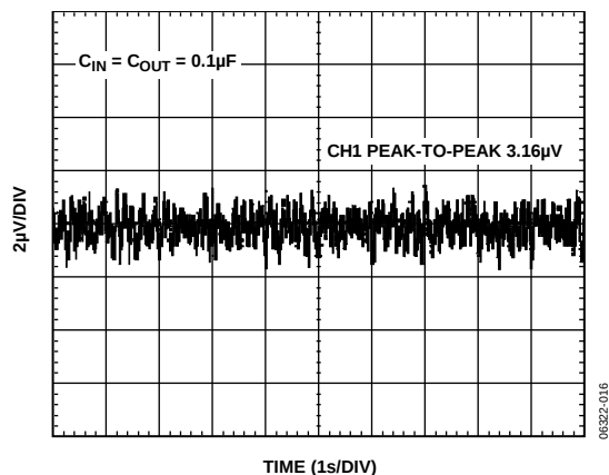
Figure 16. 0.1 Hz to 10 Hz Noise, V_{OUT} = 0.5\text{ V}
