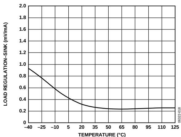
Figure 18. Load Regulation (Sink) vs. Temperature, V_{OUT} = 1\text{ V}
