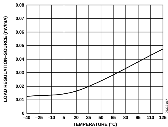
Figure 17. Load Regulation (Source) vs. Temperature, V_{OUT} = 1\text{ V}
