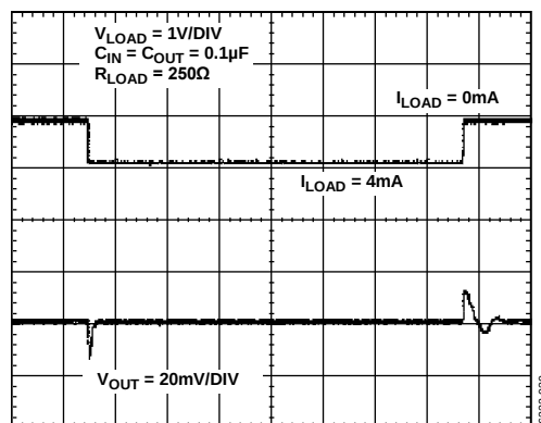
Figure 30. Load Transient Response (Source), V_{OUT} = 1\text{ V}
