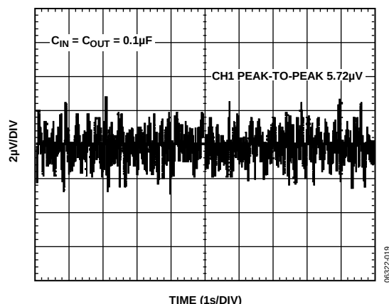
Figure 19. 0.1 Hz to 10 Hz Noise, V_{OUT} = 1\text{ V}
