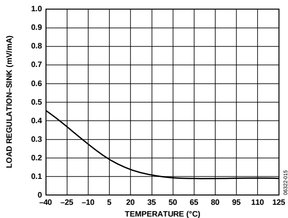
Figure 15. Load Regulation (Sink) vs. Temperature, V_{OUT} = 0.5\text{ V}
