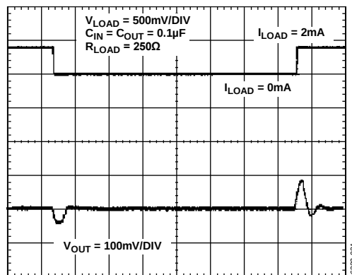
Figure 31. Load Transient Response (Sink), V_{OUT} = 1\text{ V}
