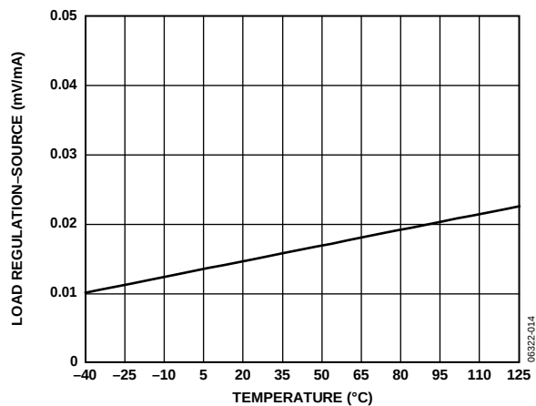
Figure 14. Load Regulation (Source) vs. Temperature, V_{OUT} = 0.5\text{ V}
