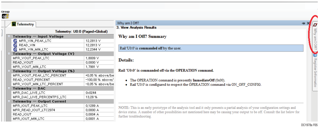
Figure 5. “Why am I Off?” tool in the LTpowerPlay GUI
