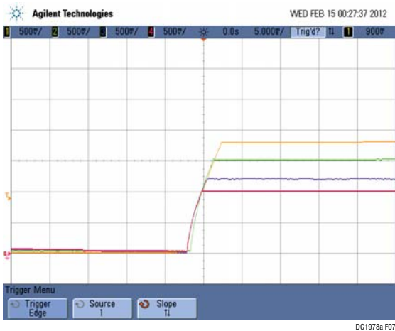
Figure 7. Tracking Supplies Up with DC1978A
