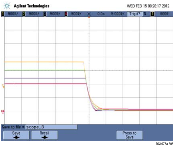
Figure 8. Tracking Supplies Down with DC1978A
