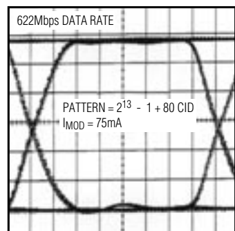
ELECTRICAL EYE DIAGRAM ( I_{MOD} = 75mA )
