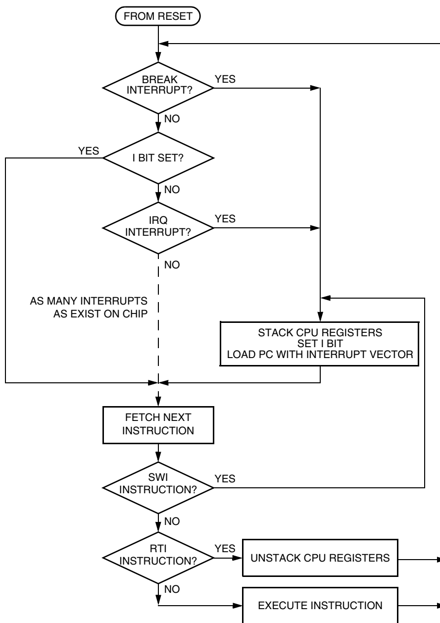
Figure 19-10. Interrupt Processing
