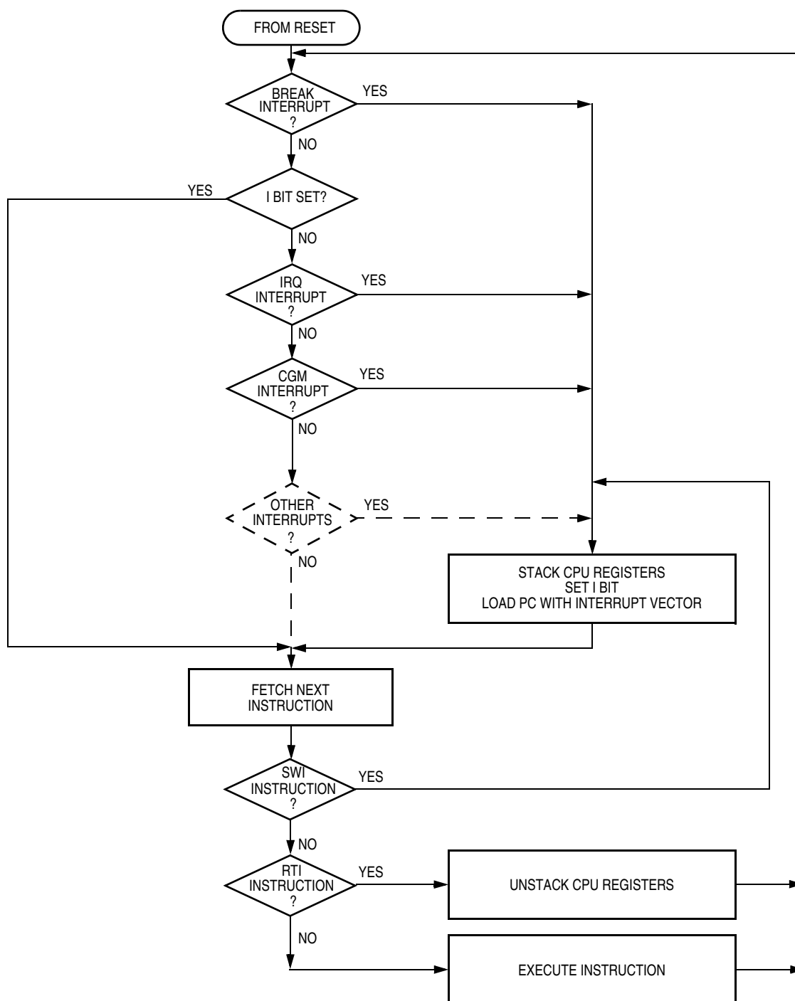
Figure 4-6. Interrupt Processing
