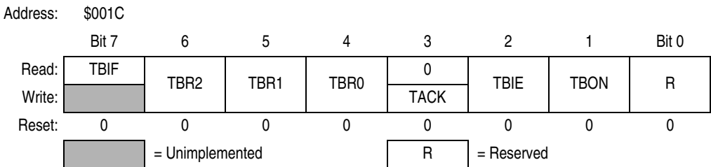
Figure 21-2. Timebase Control Register (TBCR)
