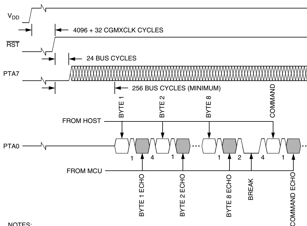
Figure 15-8. Monitor Mode Entry Timing
