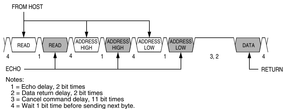
Figure 15-5. Read Transaction
