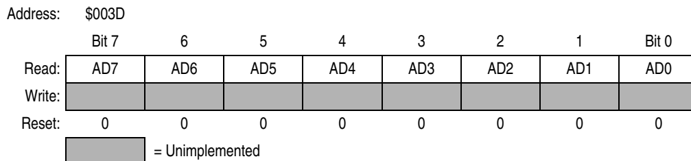
Figure 5-3. ADC Data Register (ADR)
