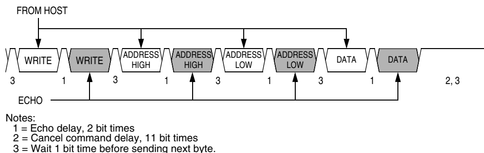
Figure 15-6. Write Transaction
