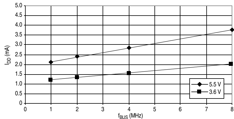
Figure 23-14. Typical Wait Mode I DD , with all Modules Disabled (–40 °C to 85 °C)
