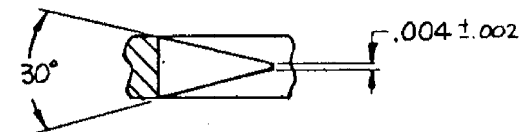
SECTION A-A ENLARGED
