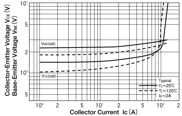
Saturation Characteristics
