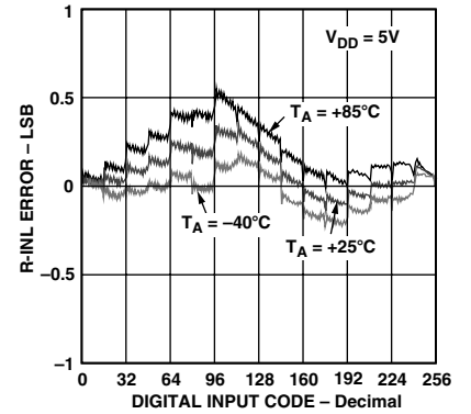
TPC 3. Resistance Step Position Nonlinearity Error vs. Code
