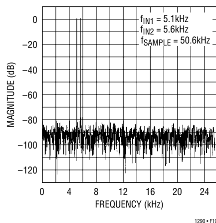
Figure 19. LTC1290 FFT Plot
