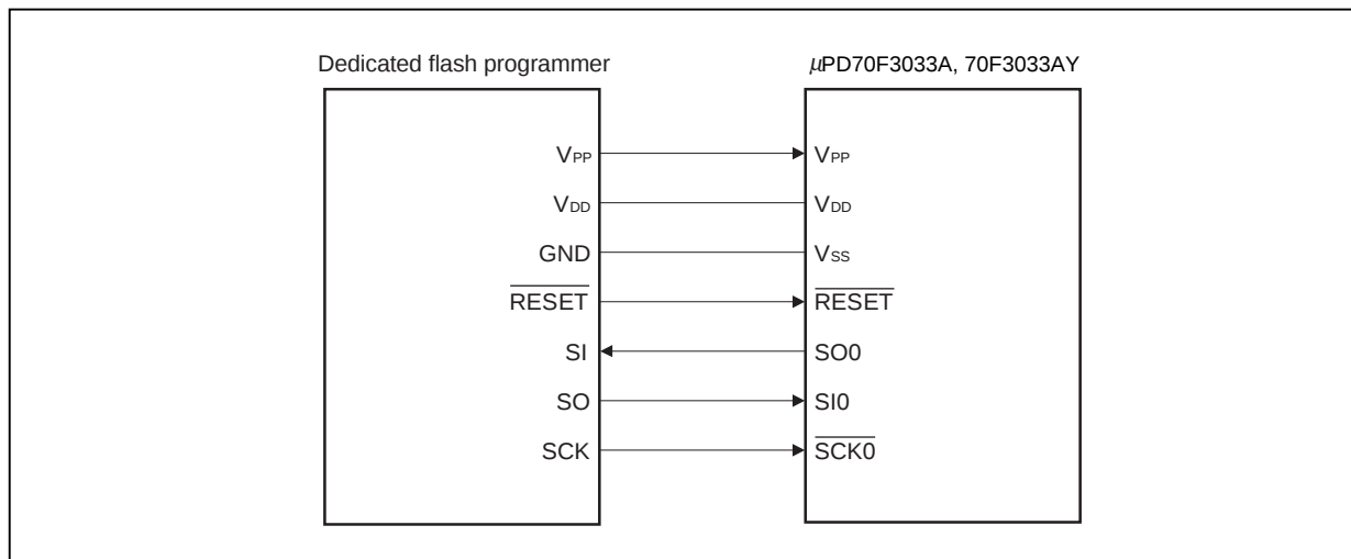
Figure 3-2. Connection of Dedicated Flash Programmer in CSI0 Mode
