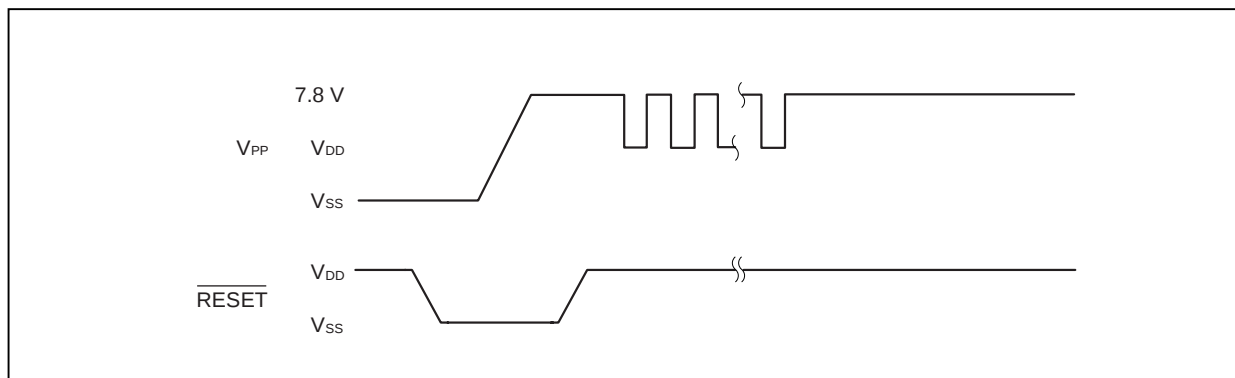
Figure 3-1. Communication Mode Selecting Format
