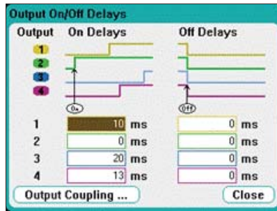
Figure 10. The Output On/Off Delays screen allows you to enter the delay times for each output. A graphical representation of the settings is shown to visually confirm your choices.
