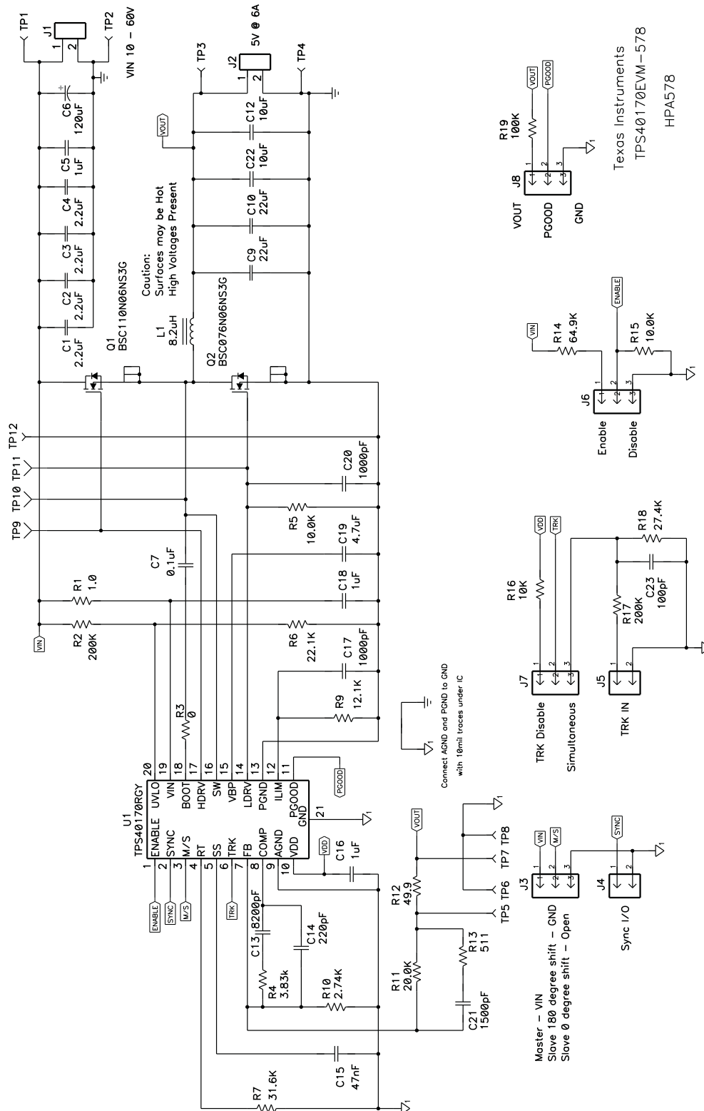
Figure 1. TPS40170EVM-578 Schematic
