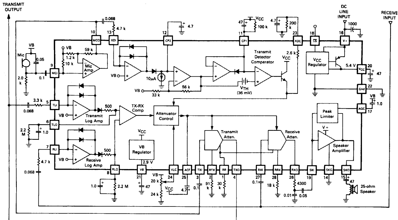
FIGURE 1 — TEST CIRCUIT
