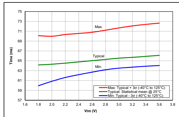
FIGURE 36-108: PWRT Period, PIC16LF18324/18344 Only
