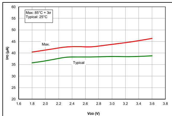
FIGURE 36-16: I PD , Fixed Voltage Reference (FVR), PIC16LF18324/18344 Only
