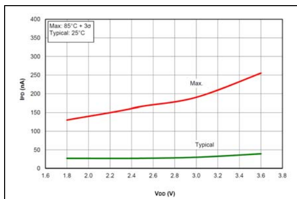
FIGURE 36-13: I PD BASE, Low-Power Sleep Mode, PIC16LF18324/18344 Only
