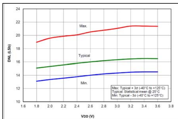
FIGURE 36-73: DAC INL Error, V_{DD} = 3.0V , PIC16LF18324/18344 Only
