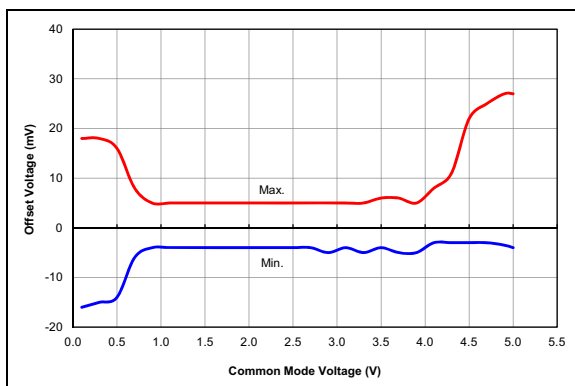
FIGURE 36-83: Comparator Offset, Normal Power Mode (CxSP = 1), VDD = 5.5V, Typical Measured Values from -40°C to 125°C, PIC16F18324/18344 Only
