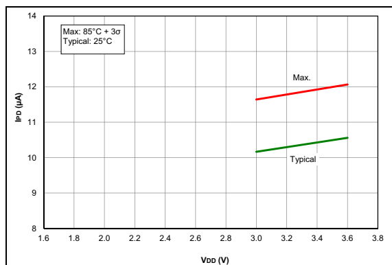
FIGURE 36-18: I PD , Brown-out Reset (BOR), BORV = 1, PIC16LF18324/18344 Only
