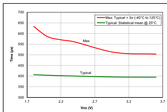
FIGURE 36-114: Wake From Sleep, LFINTOSC, PIC16LF18324/18344 Only
