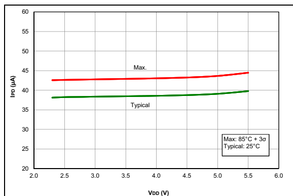
FIGURE 36-17: I PD , Fixed Voltage Reference (FVR), PIC16F18324/18344 Only
