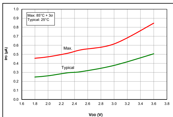
FIGURE 36-14: I PD , Watch Dog Timer (WDT), PIC16LF18324/18344 Only
