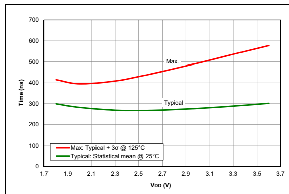
FIGURE 36-88: Comparator Response Time Rising edge, PIC16LF18324/18344 Only
