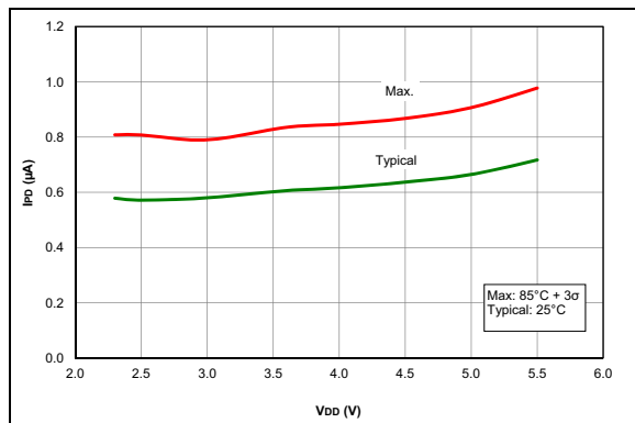
FIGURE 36-15: I PD , Watch Dog Timer (WDT), PIC16F18324/18344 Only
