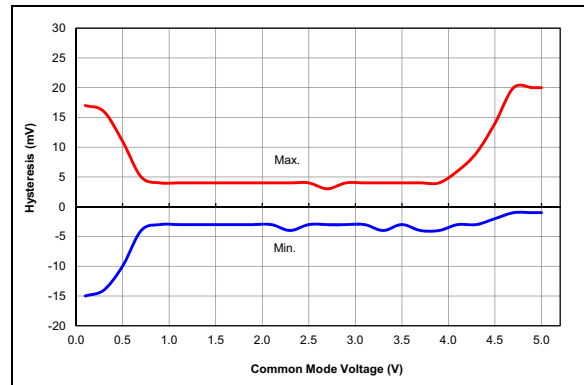
FIGURE 36-82: Comparator Offset, Normal Power Mode (CxSP = 1), VDD = 5.0V, Typical Measured Values at 25°C, PIC16F18324/18344 Only
