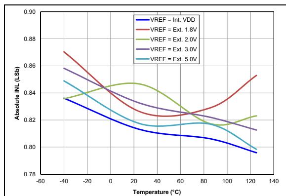
FIGURE 36-77: Absolute Value of DAC INL Error, V_{DD} = 5.0V , V_{REF} = V_{DD} , PIC16F18324/18344 Only
