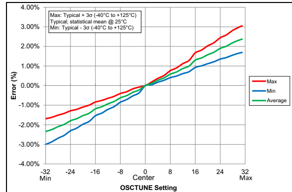
FIGURE 36-104: OSCUNE Center Frequency, PIC16LF18324/18344 Only
