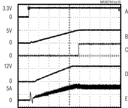
SOFT-START WAVEFORM
