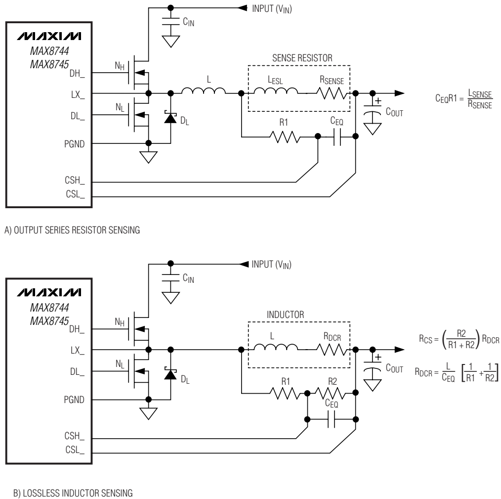
Figure 7. Current-Sense Configurations
