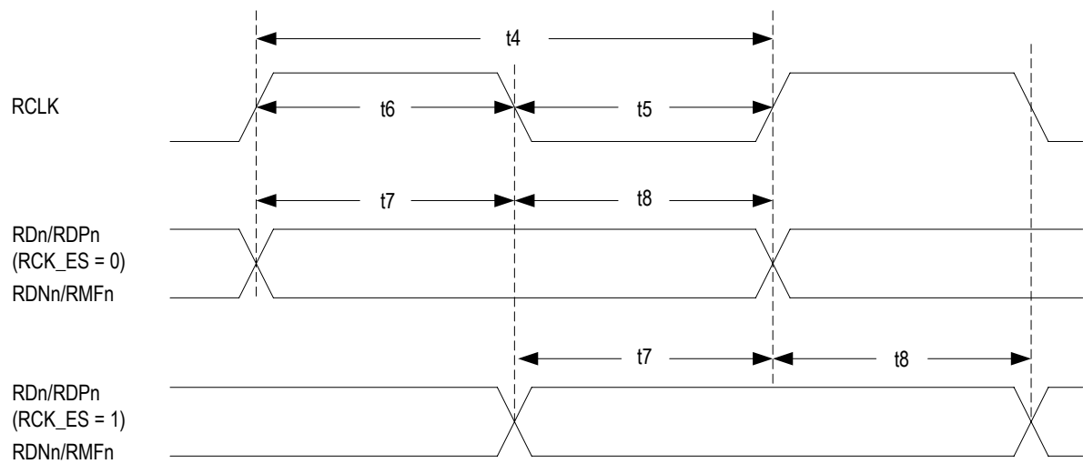
Figure-50 Receive Clock Timing Diagram
