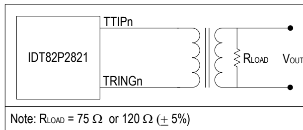
Figure-16 E1 Waveform Template Measurement Circuit
