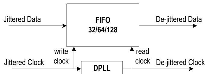
Figure-21 Jitter Attenuator
