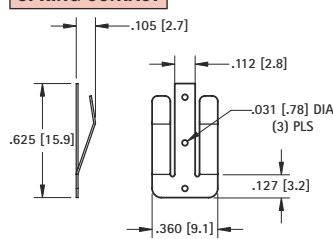
DWG. 2 MATERIAL: .010 (.25) Phosphor Bronze
