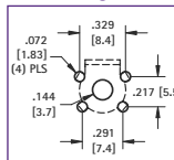
Mounting Detail
