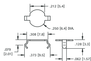
Mounting Detail
