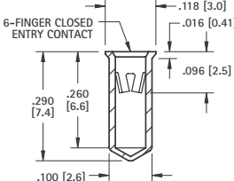
.040 (1.02) - .050 (1.27) PIN - SOLDER MOUNT
