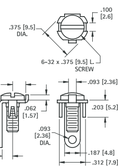
QUICK FIT
