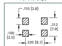
Mounting Detail For Two Clips
