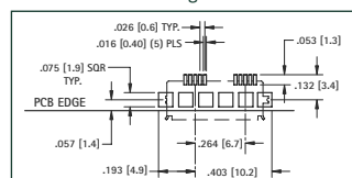
Mounting Detail
