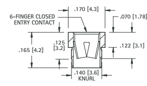
.084 (2.13) - .102 (2.6) PIN - PRESS-FIT
