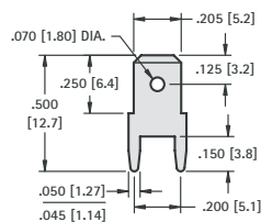
.205 (5.2) TAB
