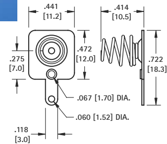
(-) NEGATIVE SPRING WITH TAB/LANCE
