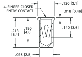
.048 (1.22) - .064 (1.63) PIN - SOLDER MOUNT
