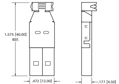
CABLE PLUG
