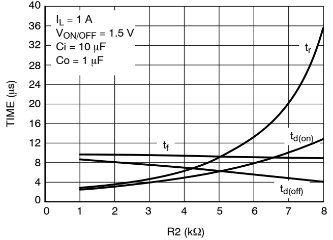
Figure 9. Switching Variation R2 @ V_{in} = 2.5\text{ V} , R_1 = 20\text{ k}\Omega
