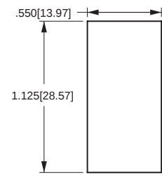
MOUNTING HOLE Panel Thickness: .020[.508] min. to .250[6.35] max.
