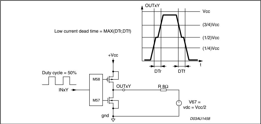
Figure 3. Test circuit 1
