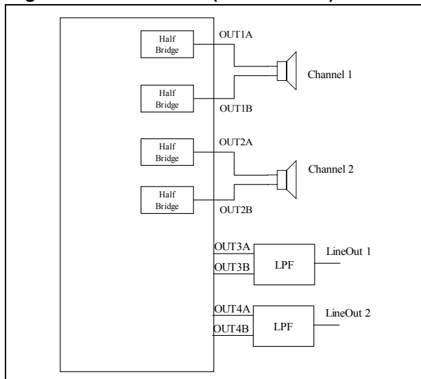
Figure 31. OCFG = 10
