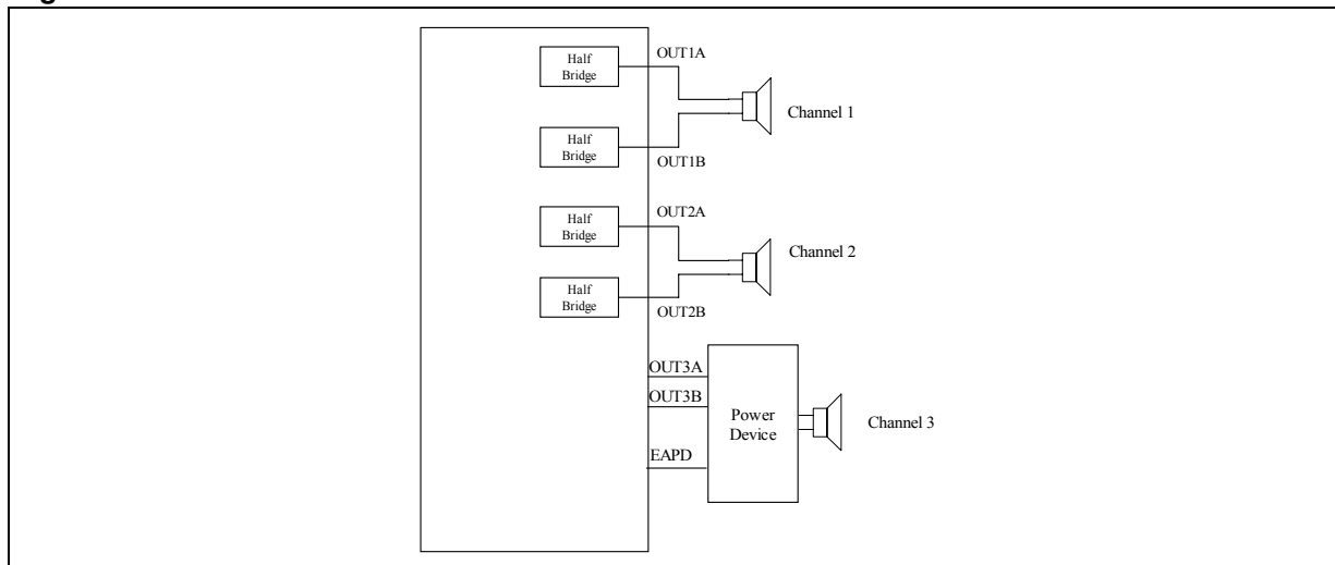
Figure 31. OCFG = 10
