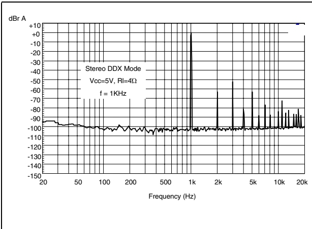
Figure 21. FFT 0 dBFS stereo DDX mode
