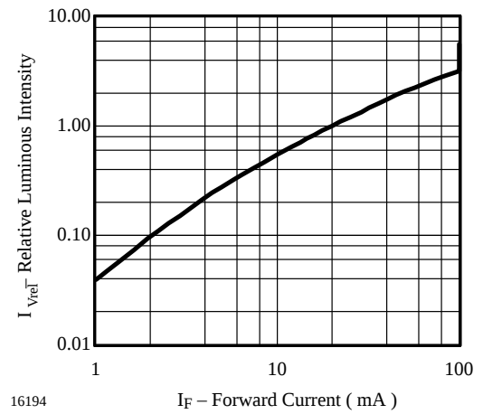
Figure 4. Relative Luminous Intensity vs. Forward Current
