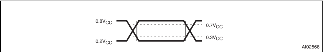
Figure 13. AC testing input/output waveforms
