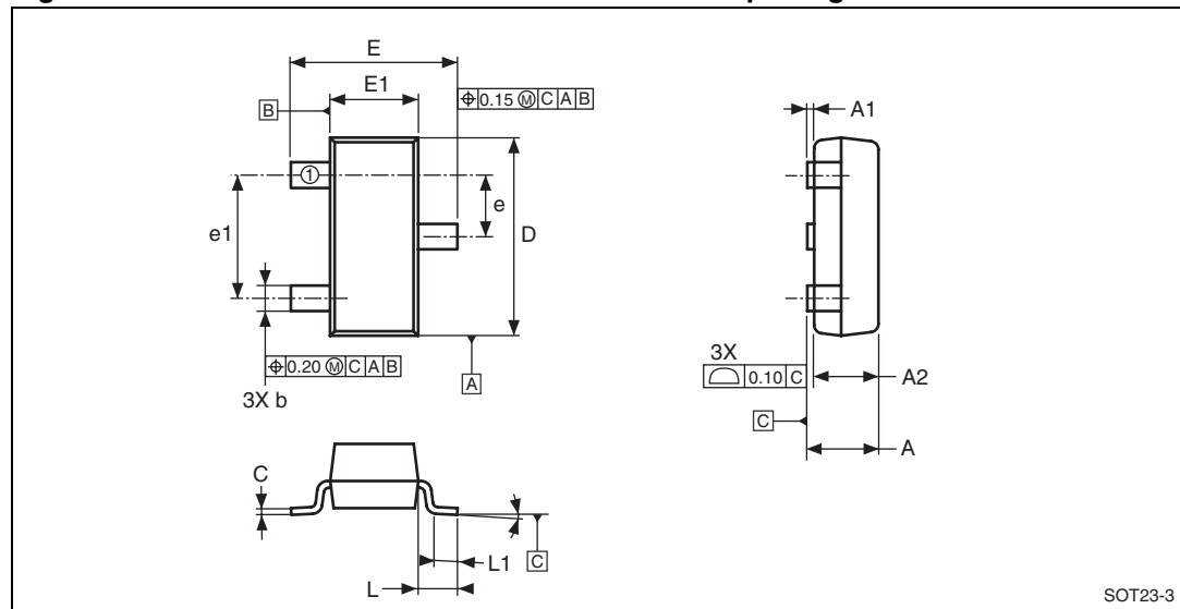
Figure 15. SOT23-3 – 3-lead small outline transistor package outline
