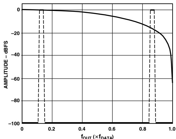
Figure 26d. No Interpolation, Modulation = f_{\text{DAC}}/8
