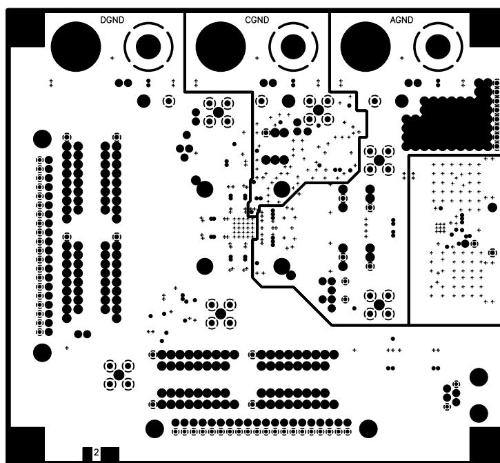
Figure 67. AD9775 Evaluation Board Layout, Layer Two (Ground Plane)
