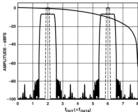
Figure 29c. 8× Interpolation, Modulation = f_{DAC}/4
