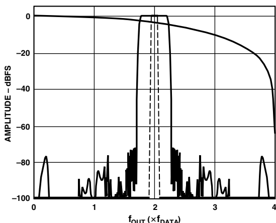
Figure 29b. 8× Interpolation, Modulation = f_{DAC}/2
