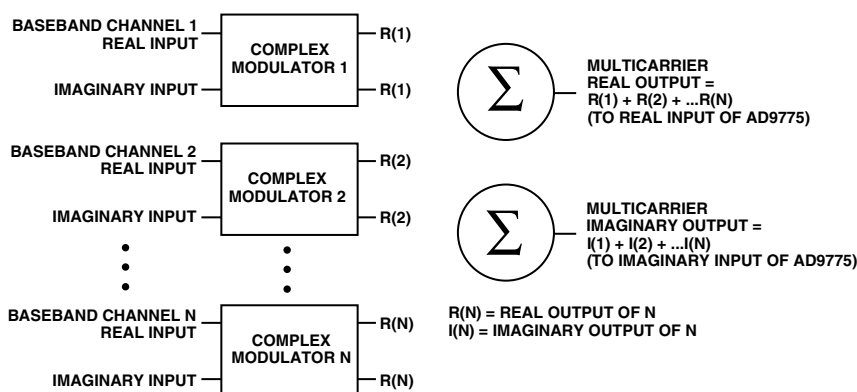
Figure 36. Synthesis of Multicarrier Complex Signal
