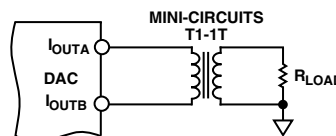
Figure 53. Transformer-Coupled Output Circuit
