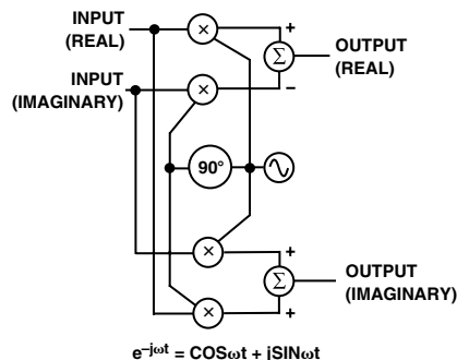
Figure 32. Implementation of a Complex Modulator
