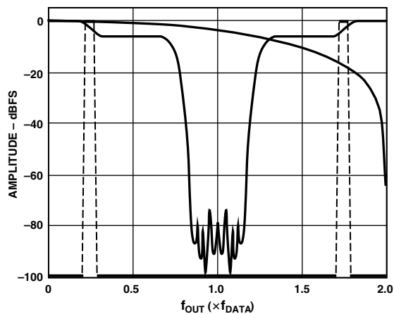
Figure 27d. 2× Interpolation, Modulation = f_{DAC}/8
