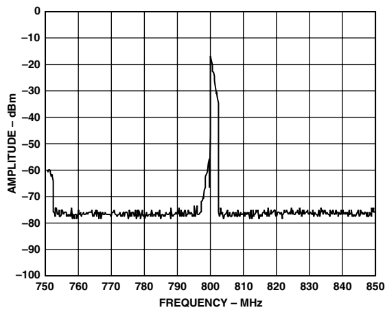
Figure 45. AD9775 Complex Output from Figure 44, Now Quadrature Modulated by AD8345 (LO = 800 MHz)
