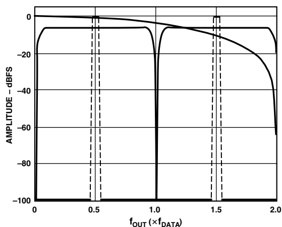
Figure 27c. 2× Interpolation, Modulation = f_{DAC}/4
