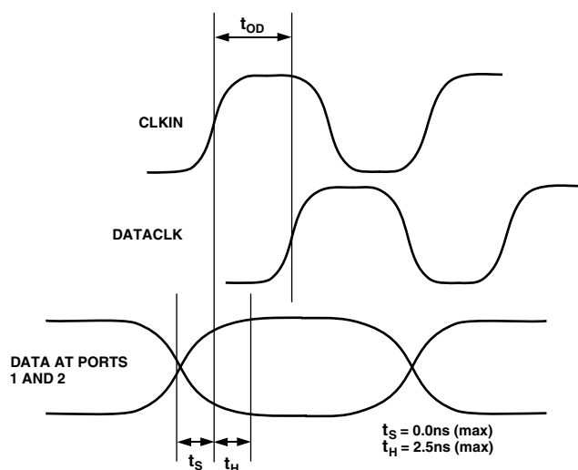
Figure 19. Timing Requirements in Two Port Input Mode, with PLL Enabled
