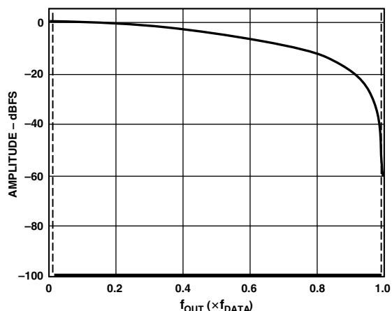
Figure 26a. No Interpolation, Modulation Disabled
