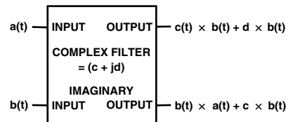
Figure 31. Realization of a Complex System
