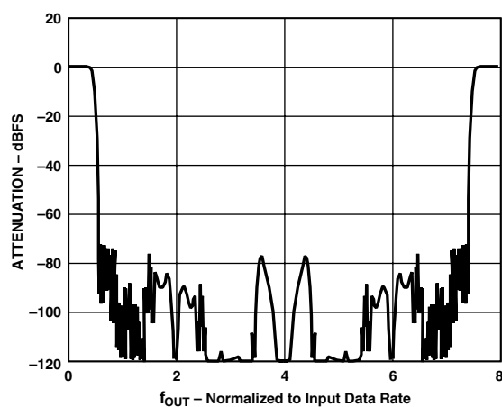
Figure 1c. 8x Interpolating Filter Response
