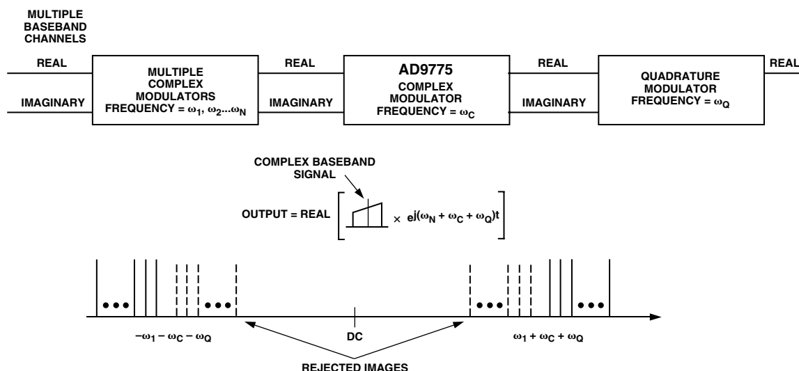
Figure 37. Image Rejection with Multicarrier Signals
