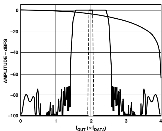
Figure 28b. 4× Interpolation, Modulation = f_{DAC}/2
