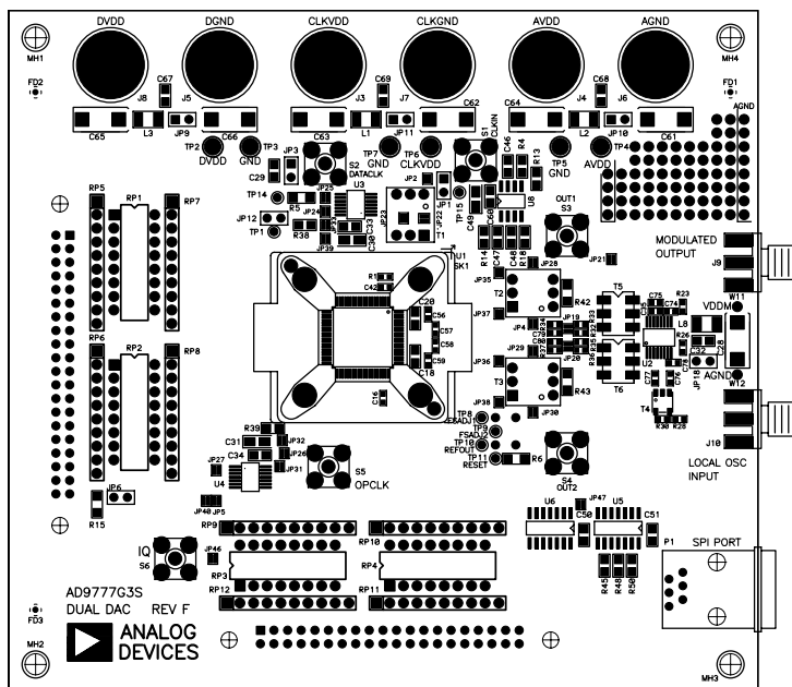
Figure 64. AD9775 Evaluation Board Components, Top Side
