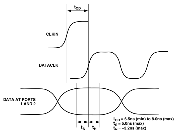
Figure 22. Timing Requirements in Two Port Input Mode with PLL Disabled
