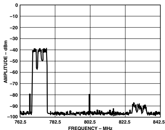
Figure 55. AD9775/AD8345 Synthesizing a Three-Carrier WCDMA Signal at an LO of 800 MHz
