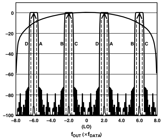
Figure 40. 8x Interpolation, Complex f_{DAC}/4 Modulation
