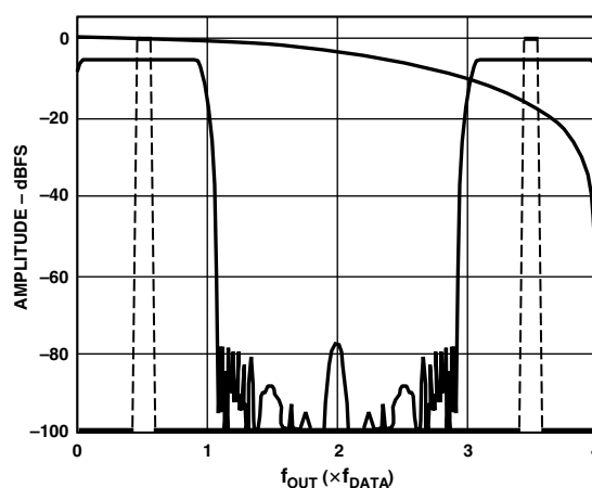
Figure 28d. 4× Interpolation, Modulation = f_{DAC}/8
