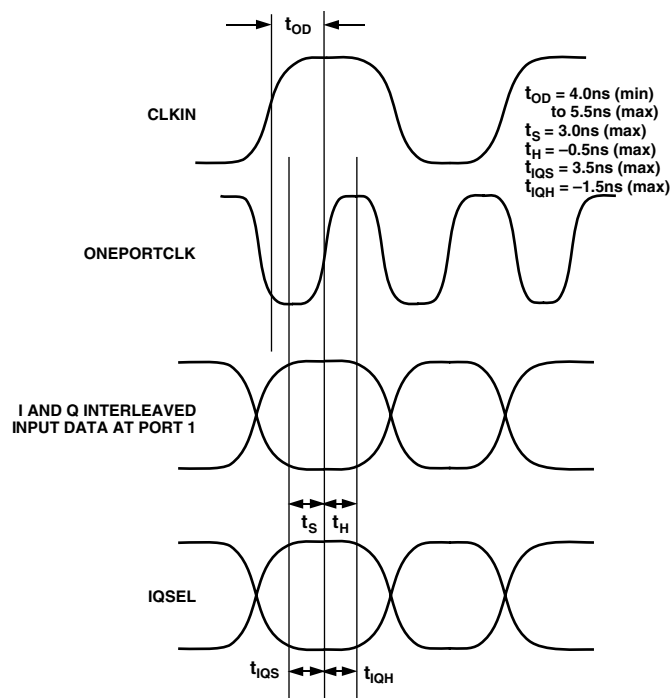
Figure 21. Timing Requirements in One Port Input Mode with the PLL Enabled
