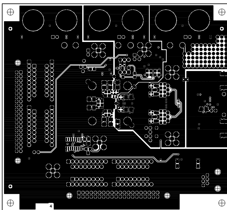
Figure 69. AD9775 Evaluation Board Layout, Layer Four (Bottom)
