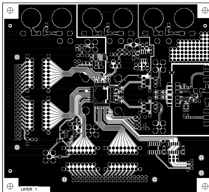
Figure 66. AD9775 Evaluation Board Layout, Layer One (Top)
