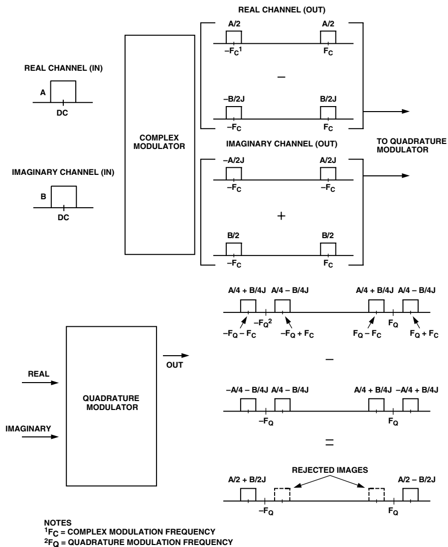
Figure 34. Two-Stage Upconversion and Resulting Image Rejection
