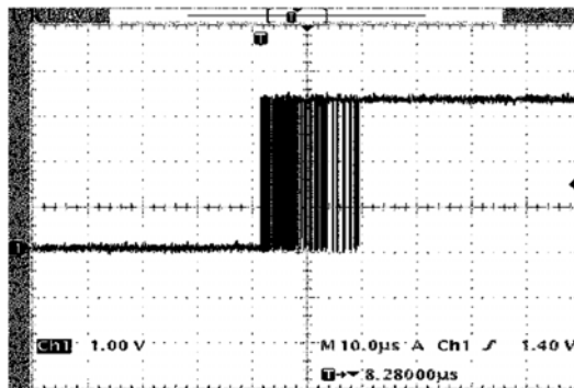
Figure 15. PLLLOCK Output Signal (Pin 8) in the Process of Locking (Typical Lock Time)
