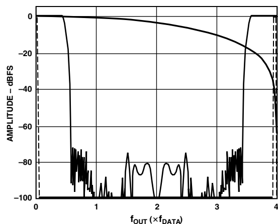
Figure 28a. 4× Interpolation, Modulation Disabled
