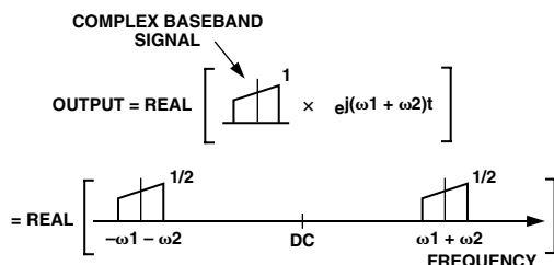
Figure 35. Two-Stage Complex Upconversion
