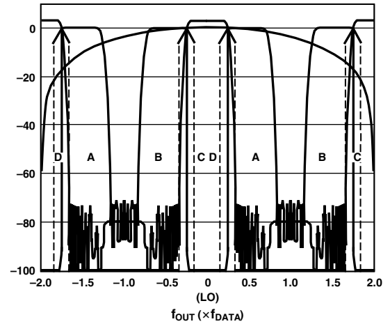
Figure 41. 2x Interpolation, Complex f_{DAC}/8 Modulation
