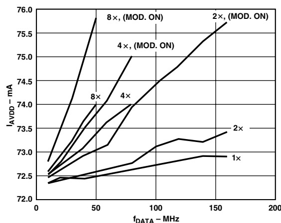
Figure 17. I_{AVDD} vs. f_{DATA} vs. Interpolation Rate, PLL Disabled
