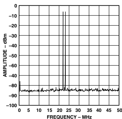
TPC 22. Two-Tone IMD Performance, f_{DATA} = 150 MSPS, Interpolation = 4x
