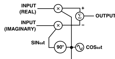
Figure 33. Quadrature Modulator
