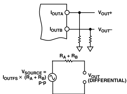
Figure 52. DAC Output Equivalent Circuit
