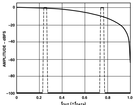
Figure 26c. No Interpolation, Modulation = f_{\text{DAC}}/4
