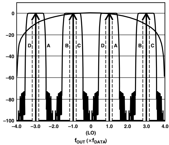
Figure 39. 4x Interpolation, Complex f_{DAC}/4 Modulation
