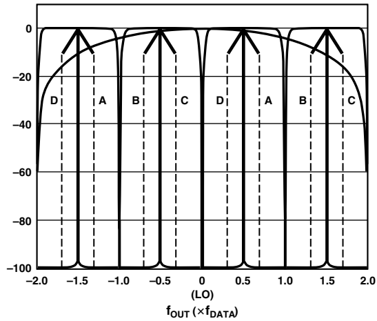
Figure 38. 2x Interpolation, Complex f_{DAC}/4 Modulation
