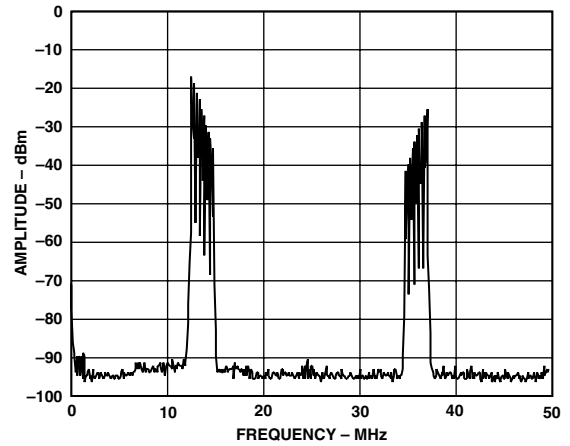
Figure 46. AD9775, Real DAC Output of Complex Input Signal Near Baseband (Positive Frequencies Only), Interpolation = 4x, Complex Modulation in AD9775 = +f_{DAC}/4
