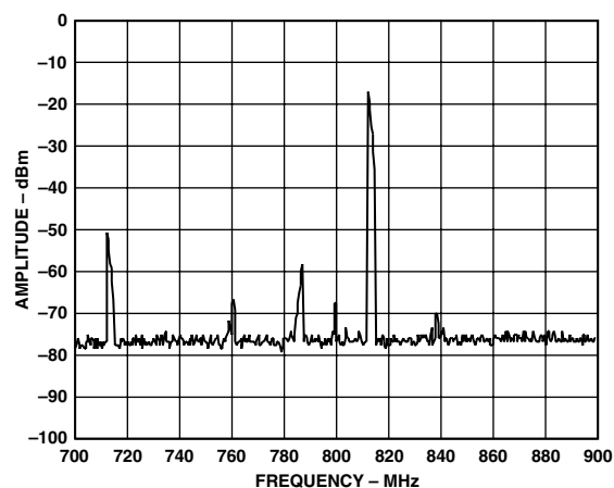
Figure 51. AD9775 Complex Output from Figure 50, Now Quadrature Modulated by AD8345 (LO = 800 MHz)
