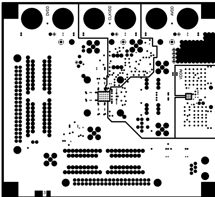
Figure 68. AD9775 Evaluation Board Layout, Layer Three (Power Plane)
