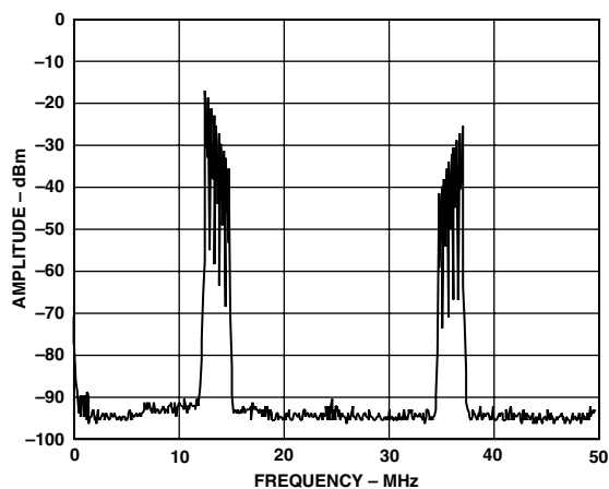
Figure 48. AD9775, Real DAC Output of Complex Input Signal Near Baseband (Negative Frequencies Only), Interpolation = 4\times , Complex Modulation in AD9775 = -f_{DAC}/4
