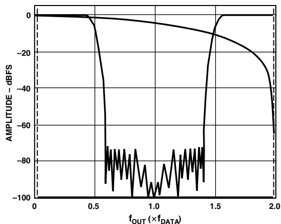
Figure 27a. 2× Interpolation, Modulation = Disabled
