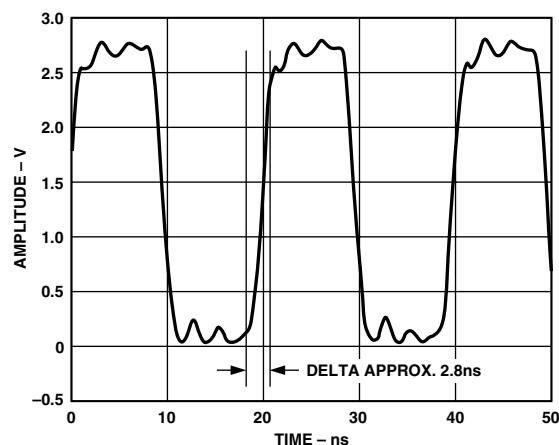
Figure 20. DATACLK Driver Capability into 330\ \Omega at 50 MHz
