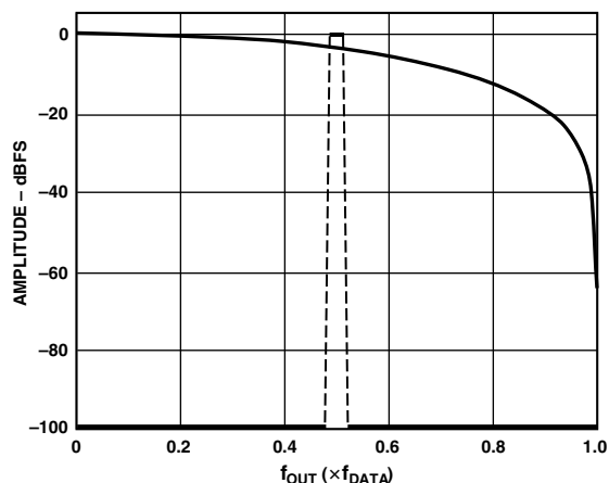
Figure 26b. No Interpolation, Modulation = f_{\text{DAC}}/2
