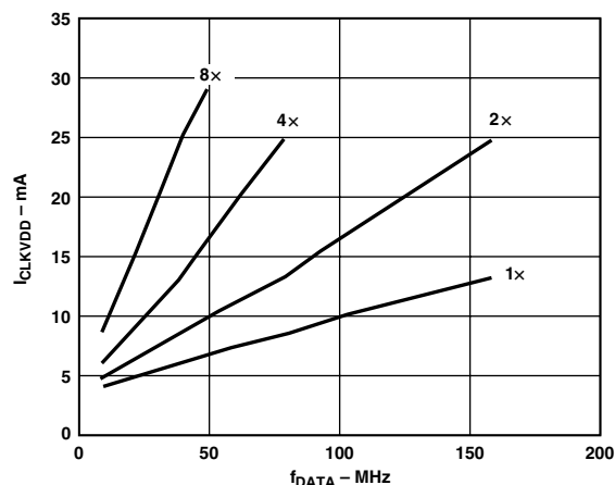
Figure 18. I_{CLKVDD} vs. f_{DATA} vs. Interpolation Rate, PLL Disabled
