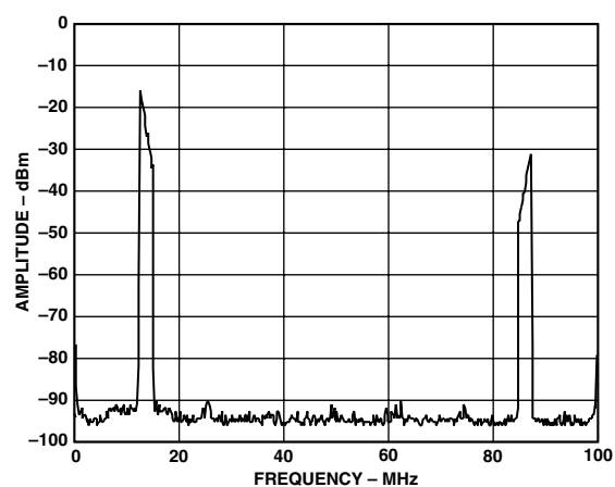
Figure 50. AD9775, Real DAC Output of Complex Input Signal Near Baseband (Positive Frequencies Only), Interpolation = 8\times , Complex Modulation in AD9775 = +f_{DAC}/8
