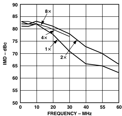
TPC 13. Third Order IMD Products vs. f_{OUT} and Interpolation Rate, 1 \times f_{DATA} = 160 MSPS 2 \times f_{DATA} = 160 MSPS 4 \times f_{DATA} = 80 MSPS 8 \times f_{DATA} = 50 MSPS
