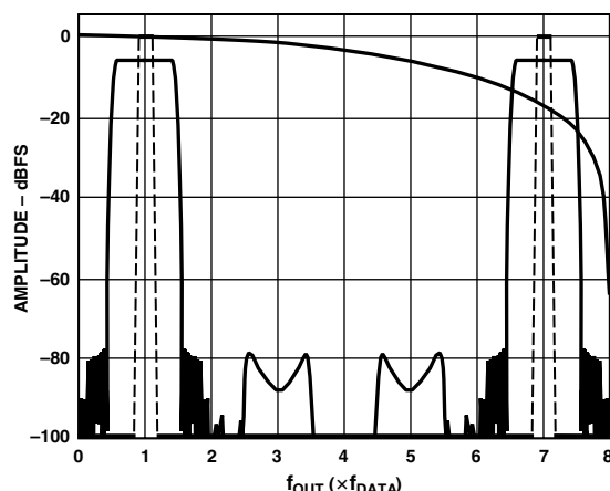
Figure 29d. 8× Interpolation, Modulation = f_{DAC}/8
