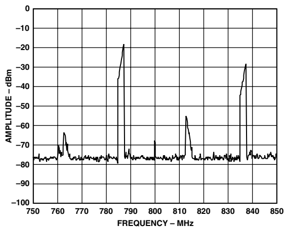
Figure 49. AD9775 Complex Output from Figure 48, Now Quadrature Modulated by AD8345 (LO = 800 MHz)
