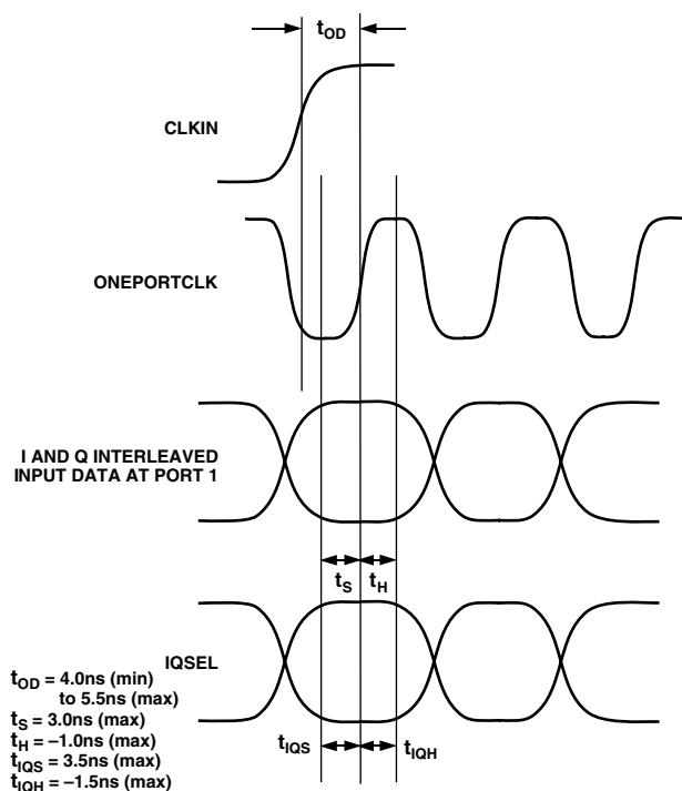
Figure 23. Timing Requirements in One Port Input Mode with PLL Disabled
