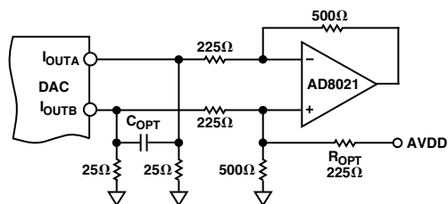
Figure 54. Op Amp-Coupled Output Circuit
