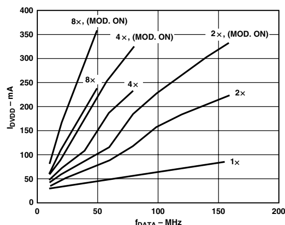
Figure 16. I_{DVDD} vs. f_{DATA} vs. Interpolation Rate, PLL Disabled
