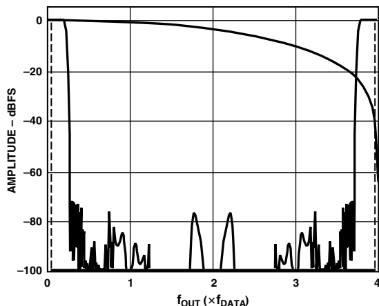
Figure 29a. 8× Interpolation, Modulation Disabled
