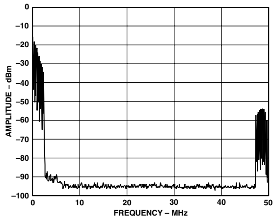
Figure 44. AD9775, Real DAC Output of Complex Input Signal Near Baseband (Positive Frequencies Only), Interpolation = 4x, No Modulation in AD9775
