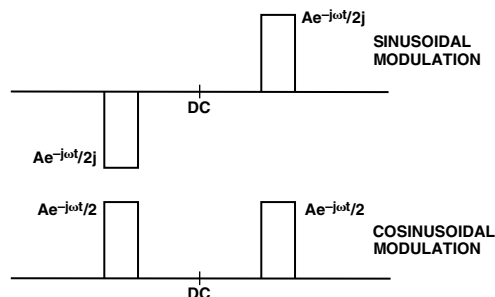
Figure 25. Baseband Signal, Amplitude Modulated with Sine and Cosine Carriers
