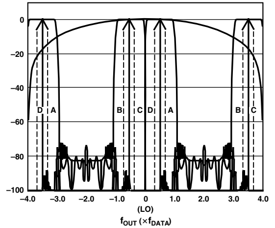
Figure 42. 4x Interpolation, Complex f_{DAC}/8 Modulation
