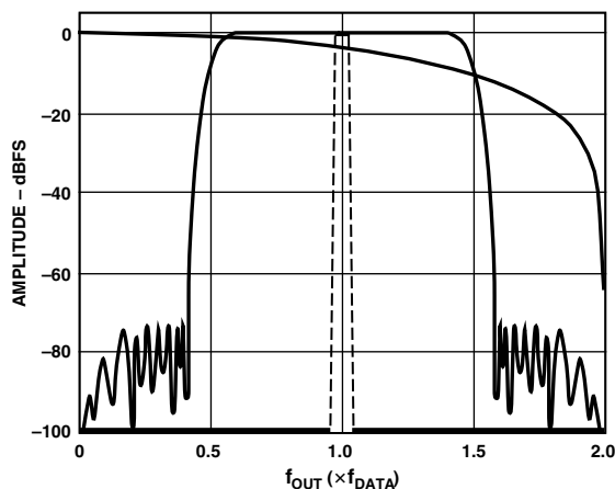
Figure 27b. 2× Interpolation, Modulation = f_{DAC}/2
