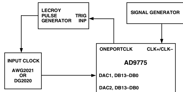
JUMPER CONFIGURATION FOR ONE PORT MODE PLL ON
