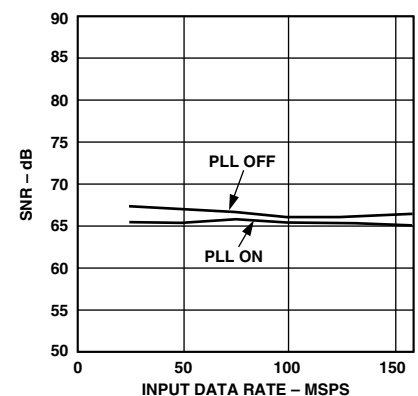
TPC 17. SNR vs. Data Rate for f_{OUT} = 5 MHz
