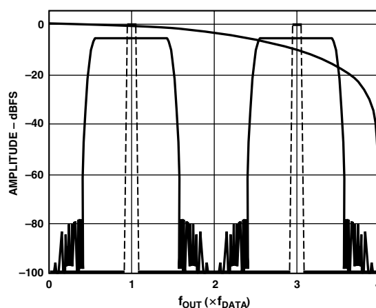
Figure 28c. 4× Interpolation, Modulation = f_{DAC}/4
