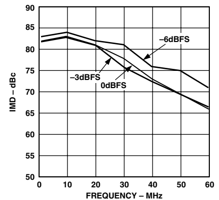
TPC 12. Third Order IMD Products vs. f_{OUT} @ f_{DATA} = 160 MSPS
