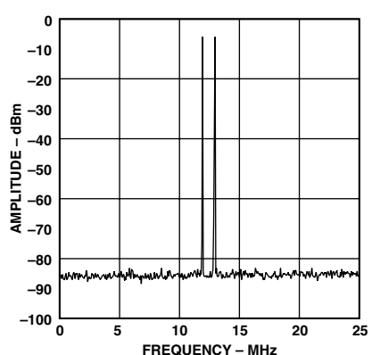
TPC 24. Two-Tone IMD Performance, f_{OUT} = 10 MHz, f_{DATA} = 50 MSPS, Interpolation = 8x
