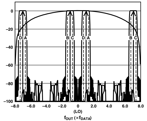
Figure 43. 8x Interpolation, Complex f_{DAC}/8 Modulation
