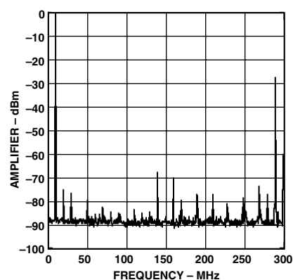
TPC 21. Single-Tone Spurious Performance, f_{OUT} = 10 MHz, f_{DATA} = 150 MSPS, Interpolation = 2x
