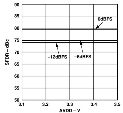
TPC 15. SFDR vs. AVDD @ f_{OUT} = 10 MHz, f_{DAC} = 320 MSPS, f_{DATA} = 160 MSPS
