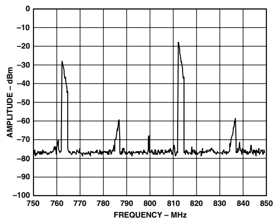
Figure 47. AD9775 Complex Output from Figure 46, Now Quadrature Modulated by AD8345 (LO = 800 MHz)
