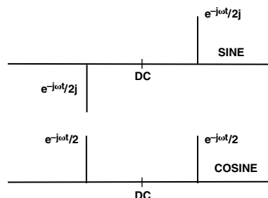
Figure 24. Real and Imaginary Components of Sinusoidal and Cosinusoidal Waveforms
