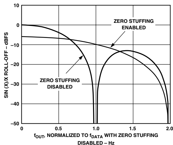
Figure 30. Effect of Zero Stuffing on DAC's \text{SIN}(x)/x Response
