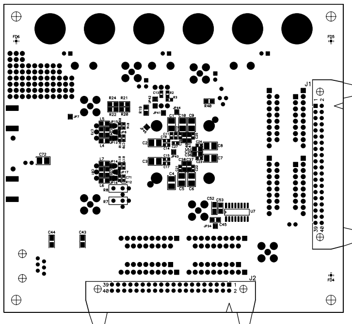
Figure 65. AD9775 Evaluation Board Components, Bottom Side
