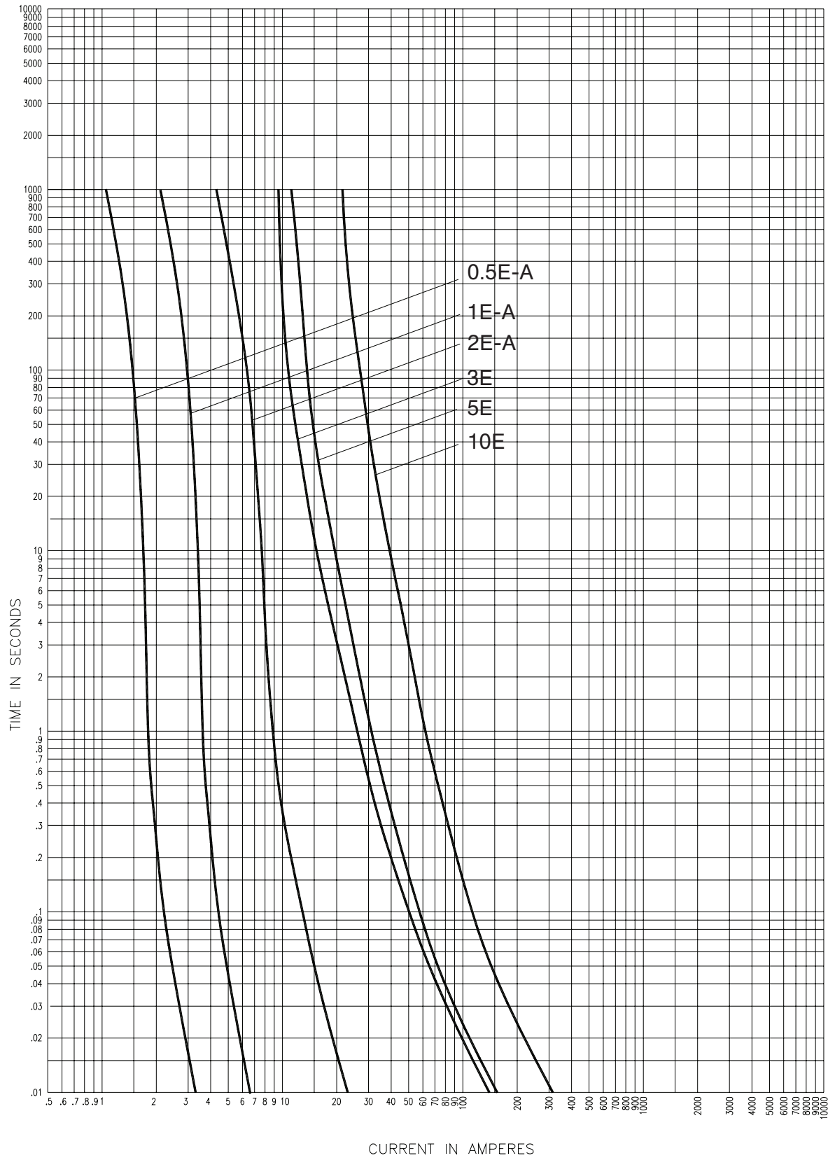
15.5 kVTime-current curves — total clearing for 15NCLPT_
