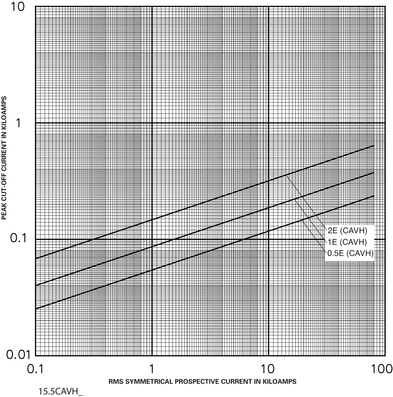
15.5 kV peak let-through curves for 15.5CAVH_
