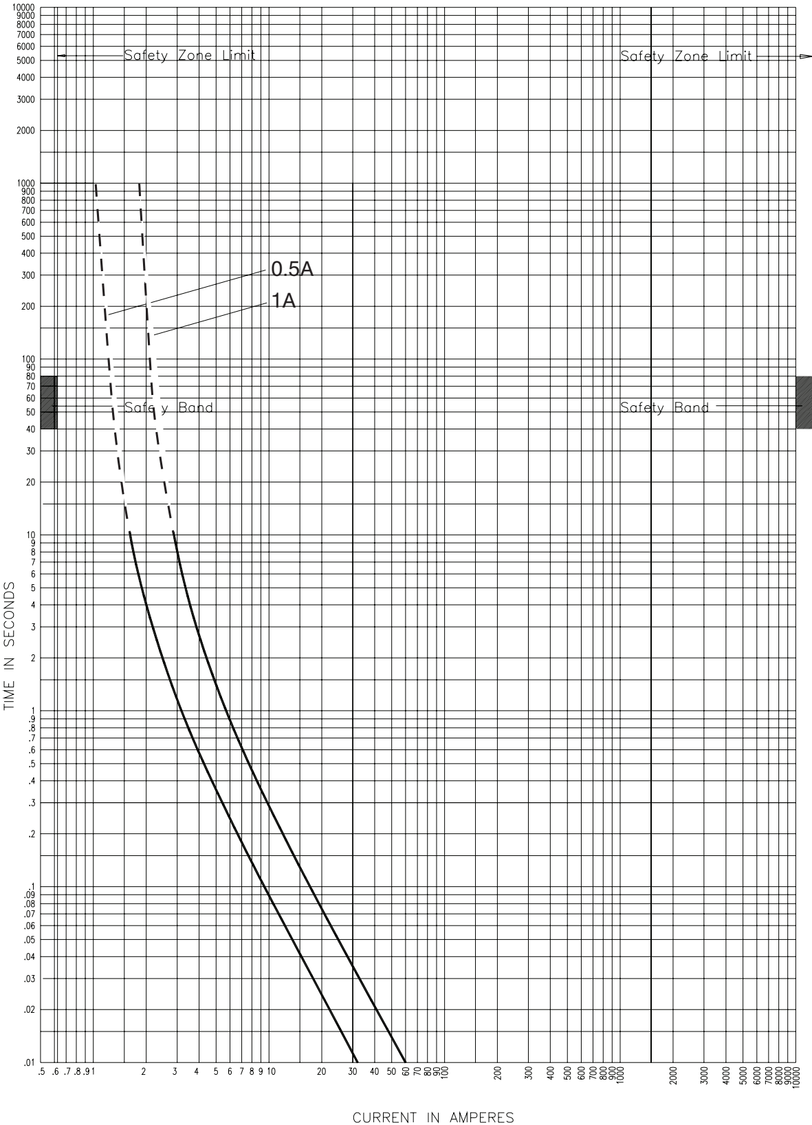
25.5 kV time-current curves — minimum melting for 25CLPT_
