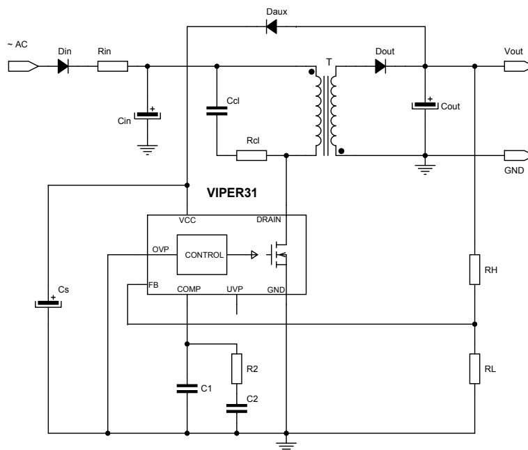
Figure 39. Flyback converter (non-isolated)
