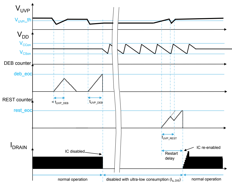
Figure 31. UVP timing
