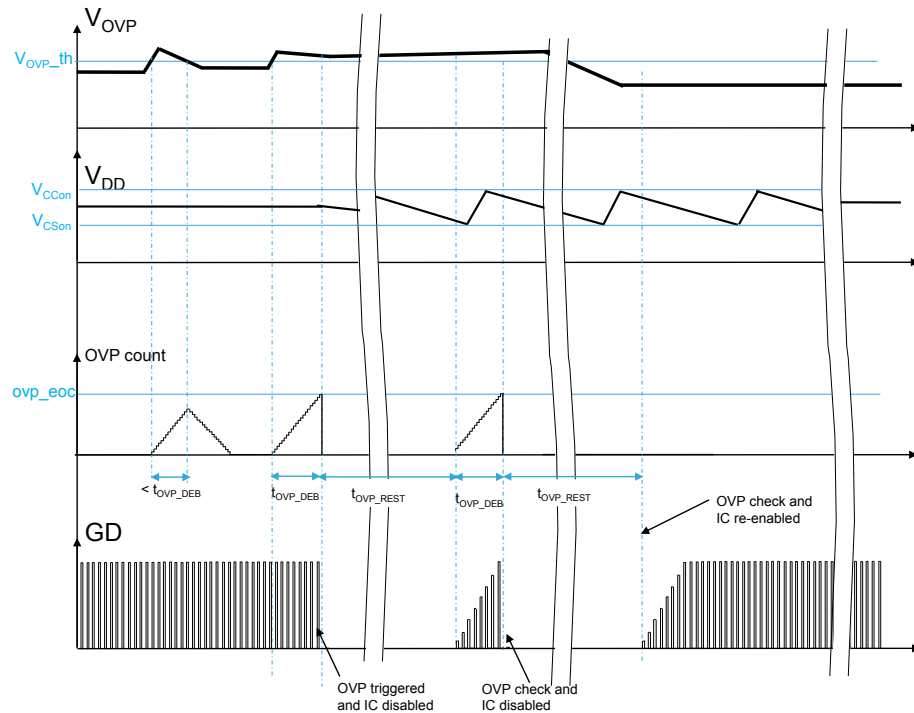
Figure 34. OVP timing
