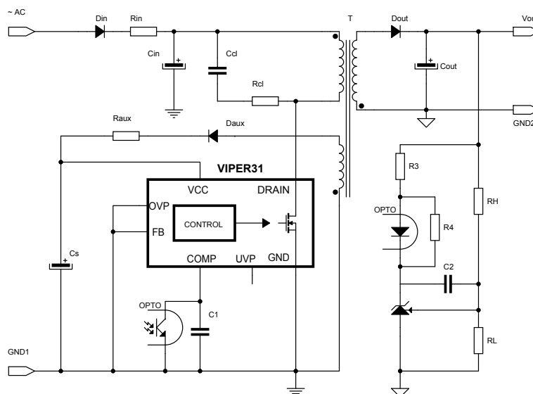
Figure 40. Flyback converter (isolated)
