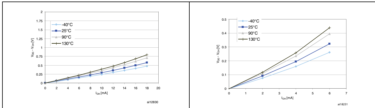
Figure 33. Typical V_{DD} - V_{OH} @ V_{DD} = 3.0 V (high sink ports) Figure 34. Typical V_{DD} - V_{OH} @ V_{DD} = 1.8 V (high sink ports)
