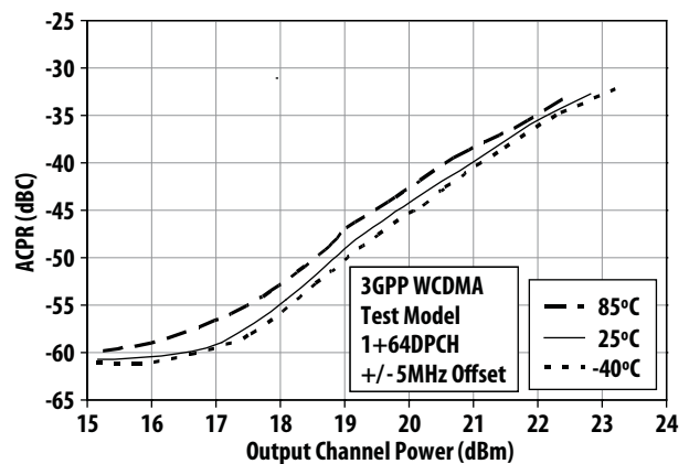
Figure 15. Over Temperature ACPR (900MHz) Vs Pout
