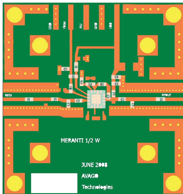
Figure 19. Demo board Layout for 400MHz to 700MHz
