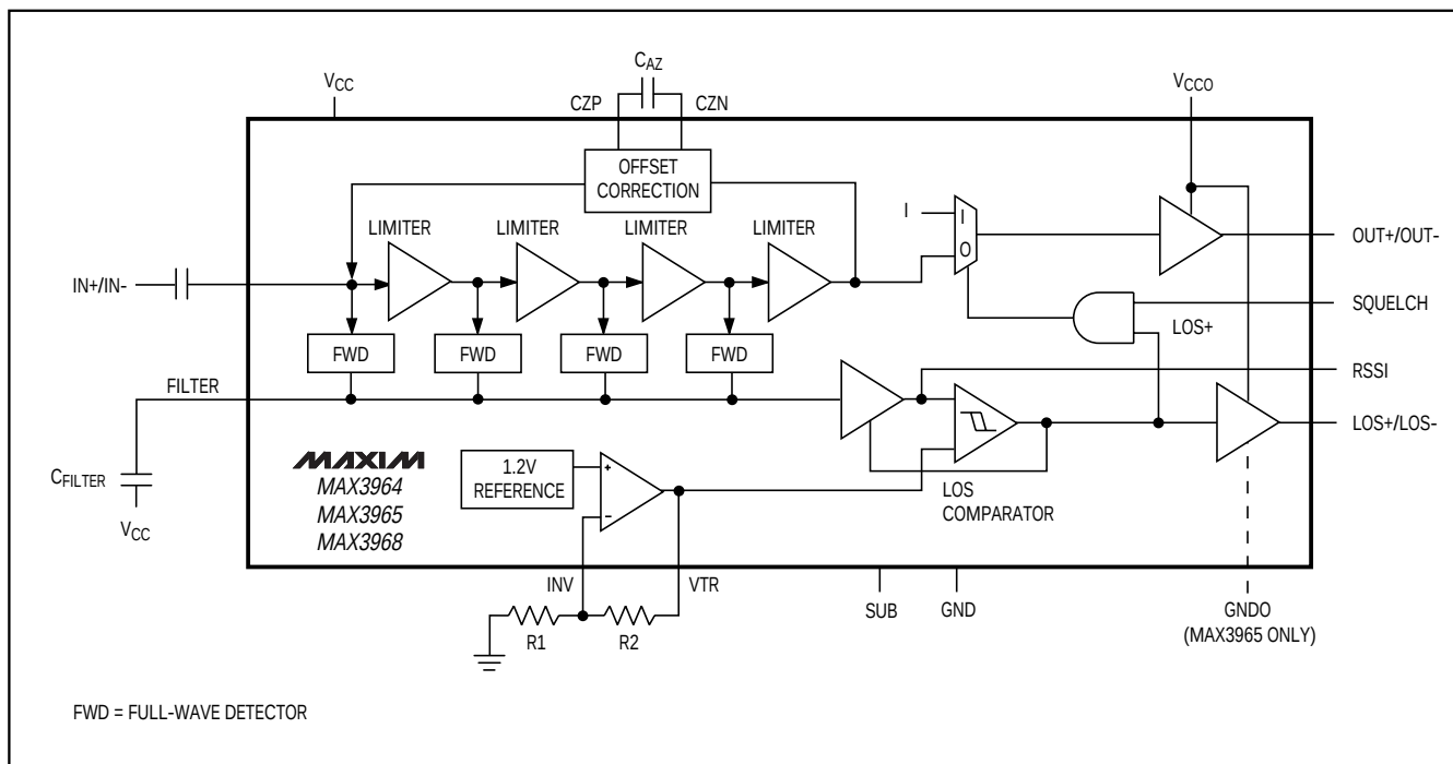
Figure 1. Functional Diagram
