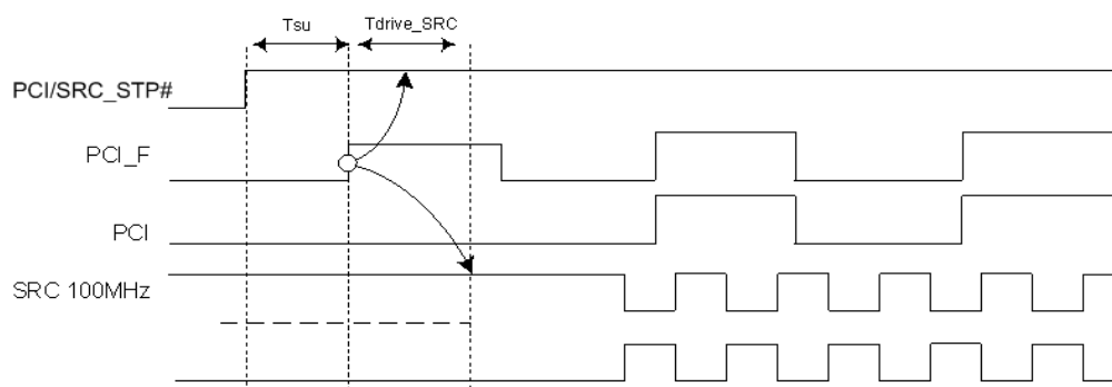
Figure 7. PCI/SRC_STP# Deassertion Waveform
