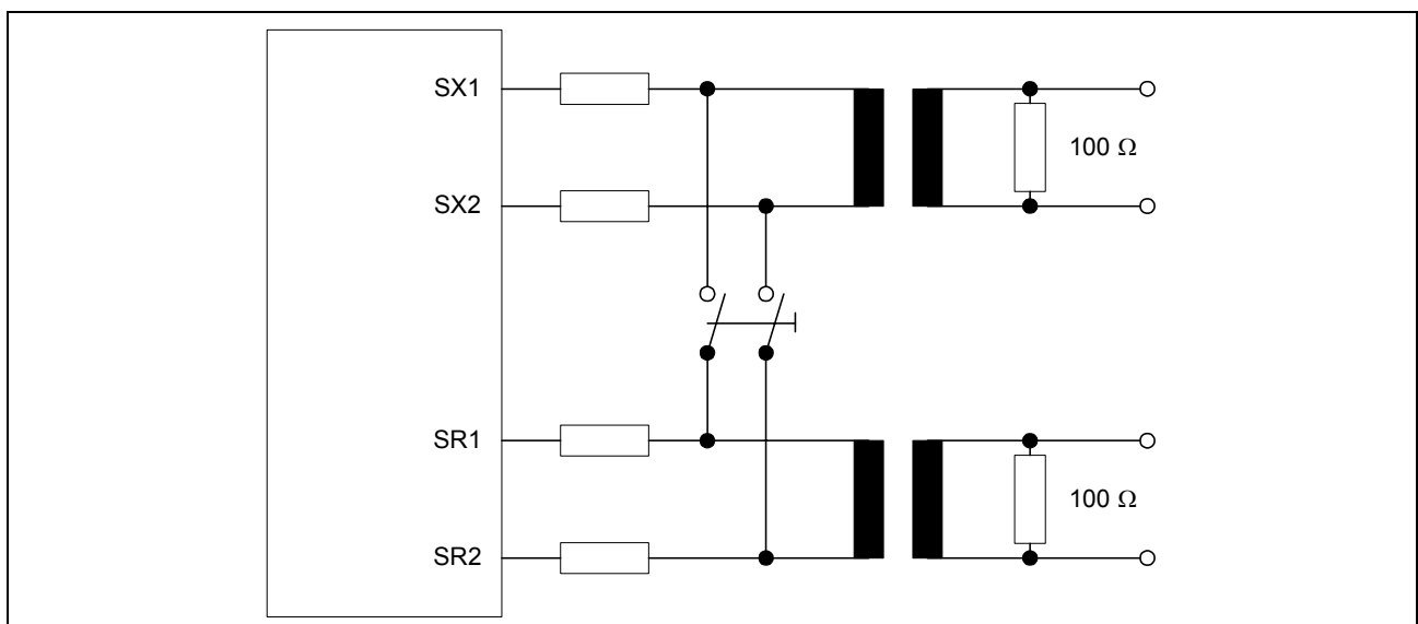
Figure 36 External Loop at the S/T-Interface
