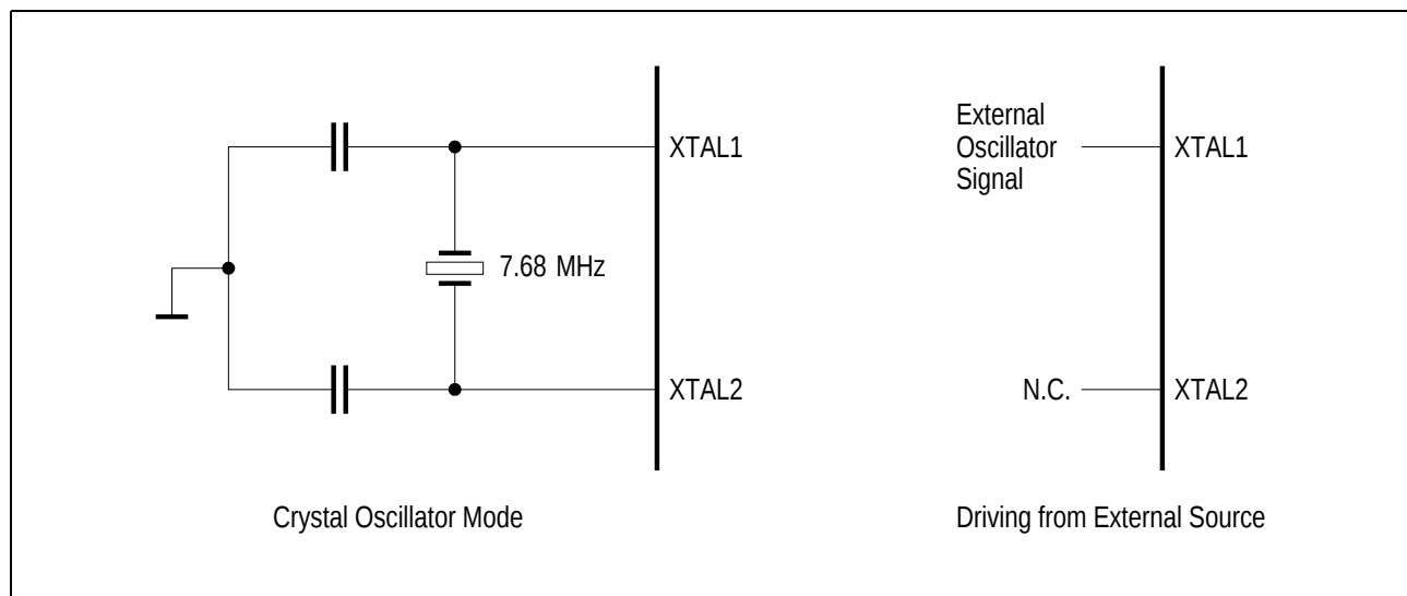
Figure 89 Oscillator Circuits
