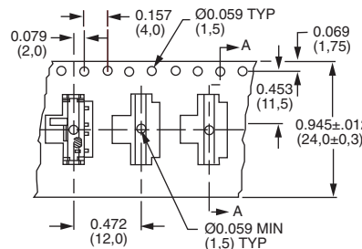
CARRIER TAPE
