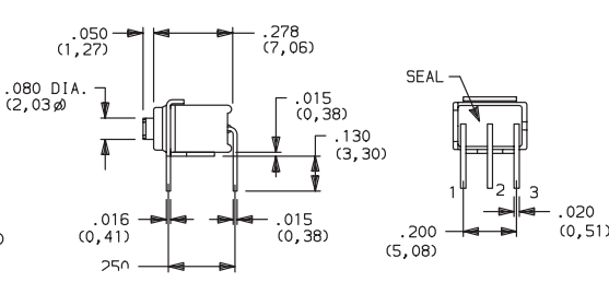
PC MOUNTING
