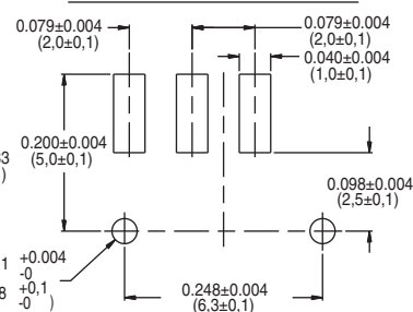
CARRIER TAPE
