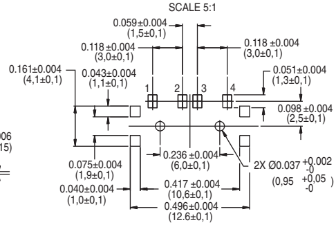
CARRIER TAPE
