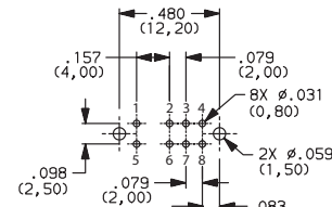
PC MOUNTING
