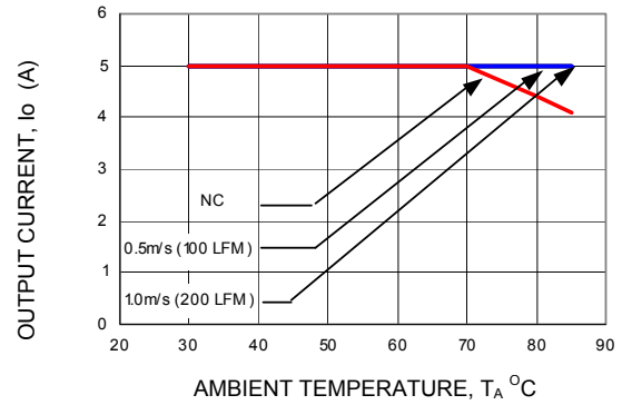
Figure 22. Derating Output Current versus Local Ambient Temperature and Airflow ( V_{in} = 3.3 Vdc, V_o = 0.75 Vdc).
