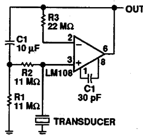
Figure 21. Amplifier for Piezoelectric Transducers
