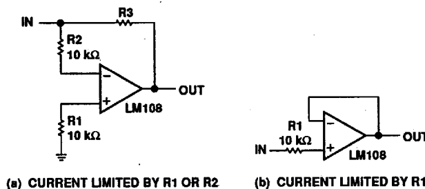
Figure 16. Input Protection
