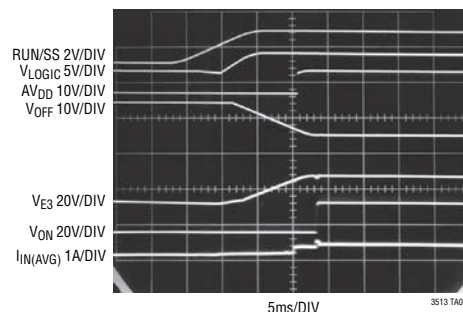
Start-Up Waveforms
