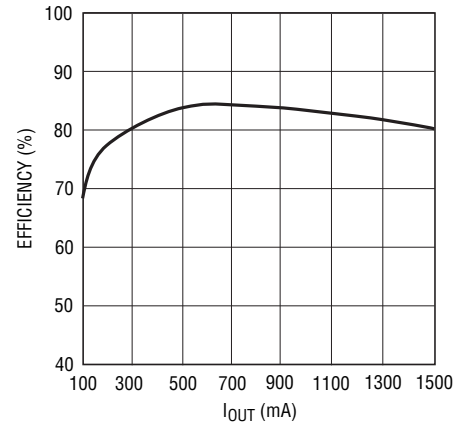
Efficiency, V_{\text{LOGIC}} = 5\text{V}
