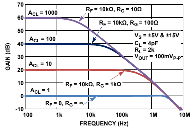
FIGURE 16. FREQUENCY RESPONSE vs CLOSED LOOP GAIN
