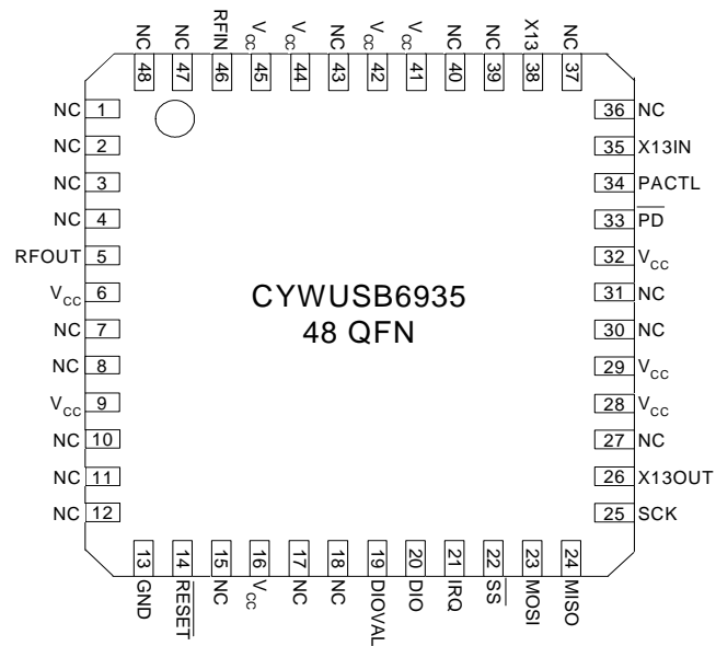
CYWUSB6935 Top View*
