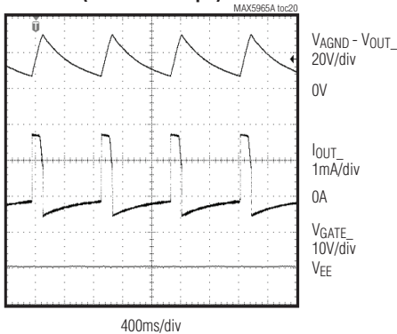
DETECTION WITH INVALID PD (25k \Omega AND 10µF)
