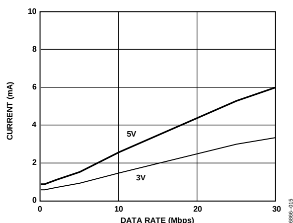
Figure 11. ADuM3211 Typical I_{DD1} or I_{DD2} Supply Current vs. Data Rate for 5 V and 3.3 V Operation
