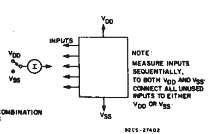
Fig. 12 — Input current test circuit.
