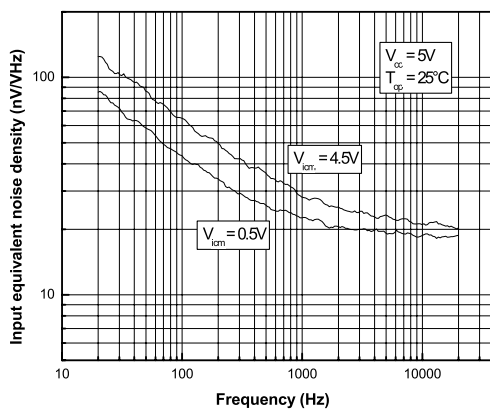
Figure 16. Noise vs. frequency
