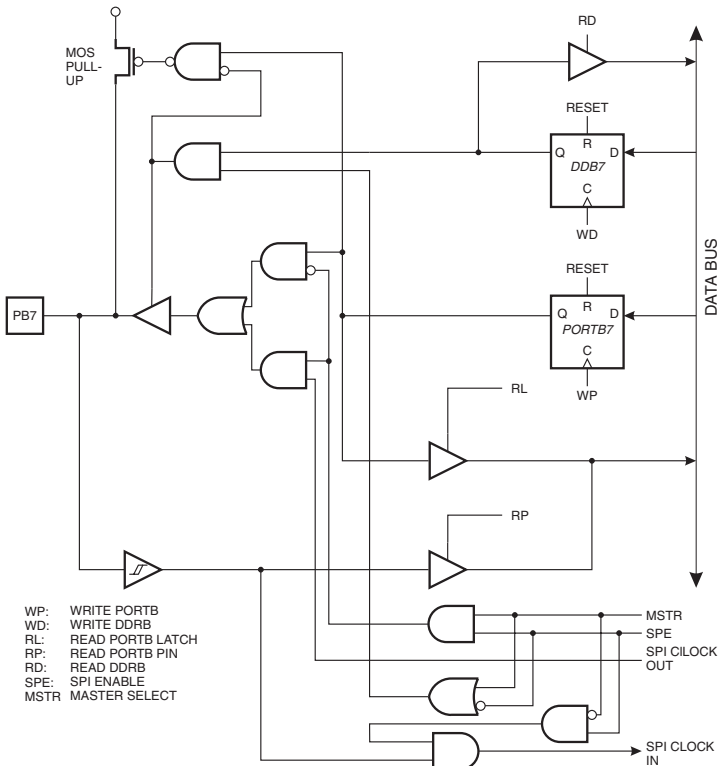
Figure 62. Port B Schematic Diagram (Pin PB7)
