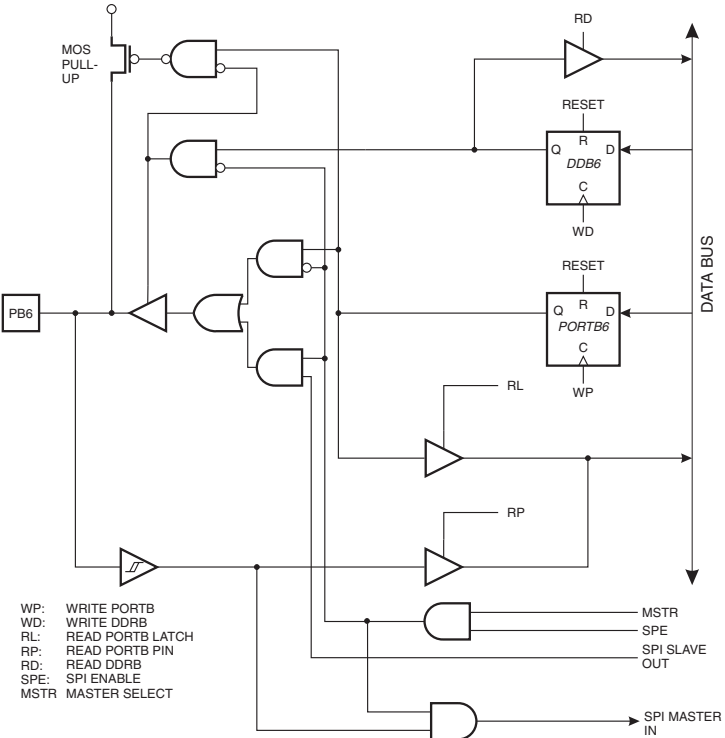
Figure 61. Port B Schematic Diagram (Pin PB6)
